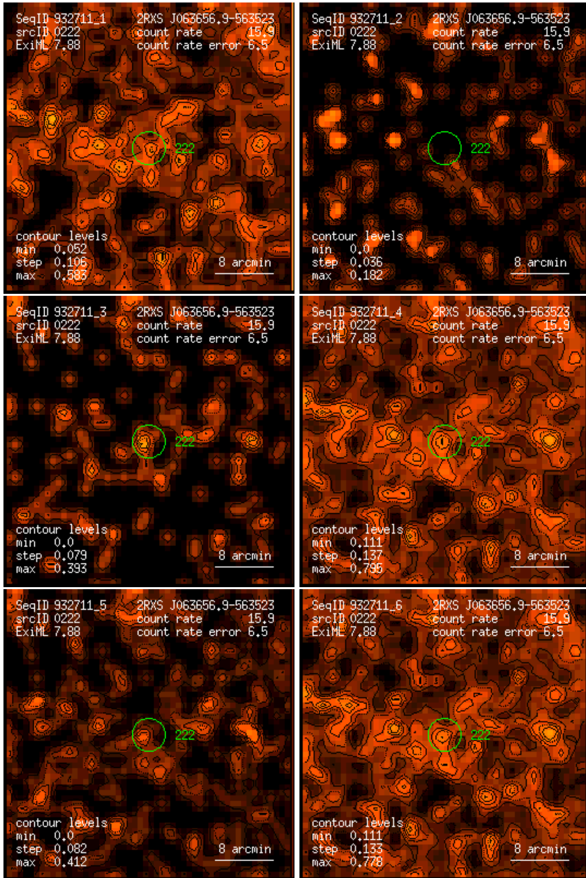
Figure 222: RASS 932711: detection 0222: band rate images, Gaussian filter: (1) PSPC channels 11 – 41, (2) 52 – 90, (3) 91 – 201, (4) 11 – 235, (5) 52 – 201, (6) 11 – 201. Broad band rates in counts/ks. Band rate contour levels in counts/ks/arcmin 2 .
