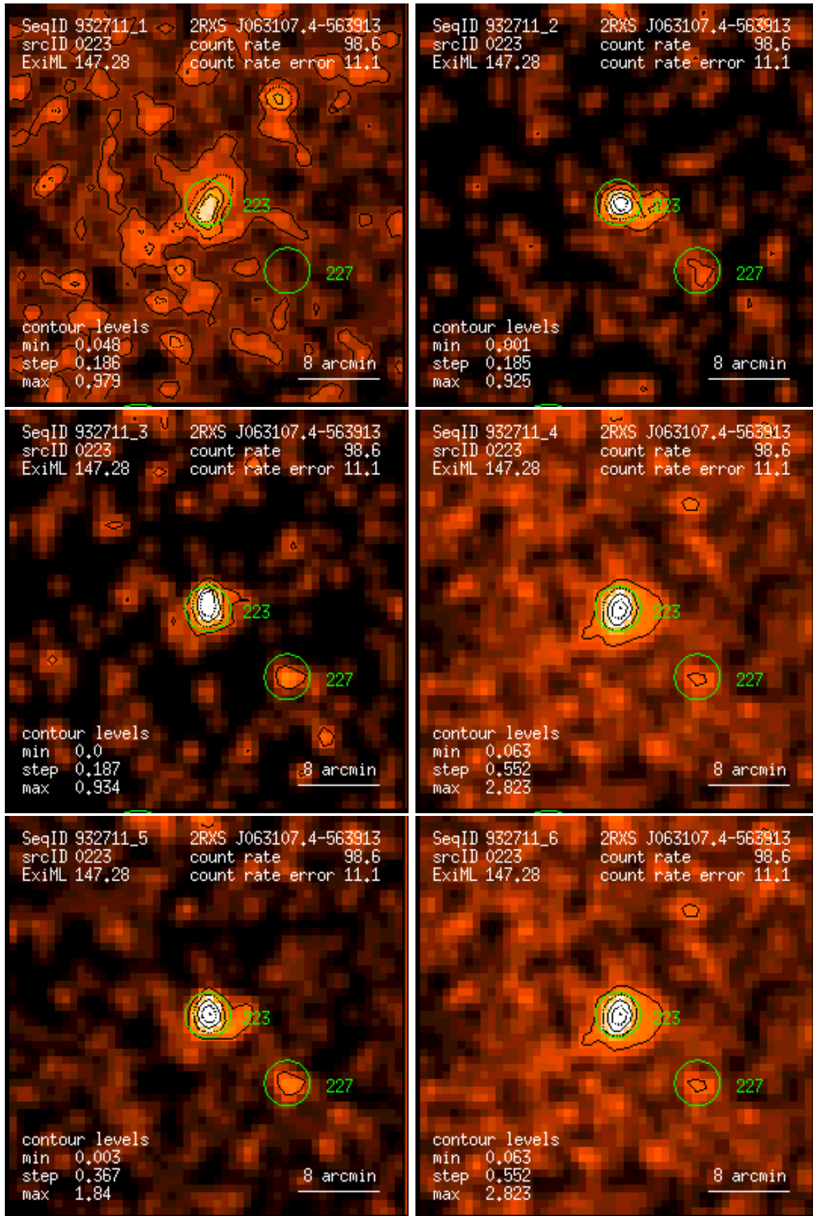
Figure 223: RASS 932711: detection 0223: band rate images, Gaussian filter: (1) PSPC channels 11 – 41, (2) 52 – 90, (3) 91 – 201, (4) 11 – 235, (5) 52 – 201, (6) 11 – 201. Broad band rates in counts/ks. Band rate contour levels in counts/ks/arcmin 2 .
