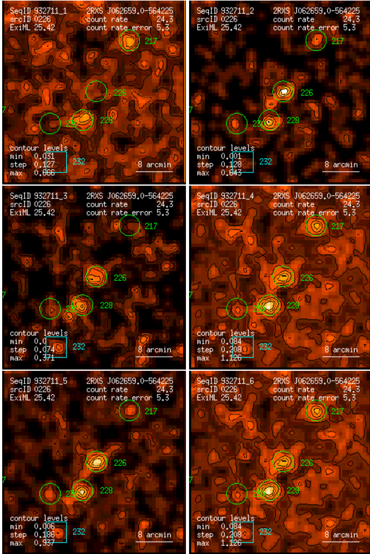
Figure 226: RASS 932711: detection 0226: band rate images, Gaussian filter: (1) PSPC channels 11 – 41, (2) 52 – 90, (3) 91 – 201, (4) 11 – 235, (5) 52 – 201, (6) 11 – 201. Broad band rates in counts/ks. Band rate contour levels in counts/ks/arcmin 2 .
