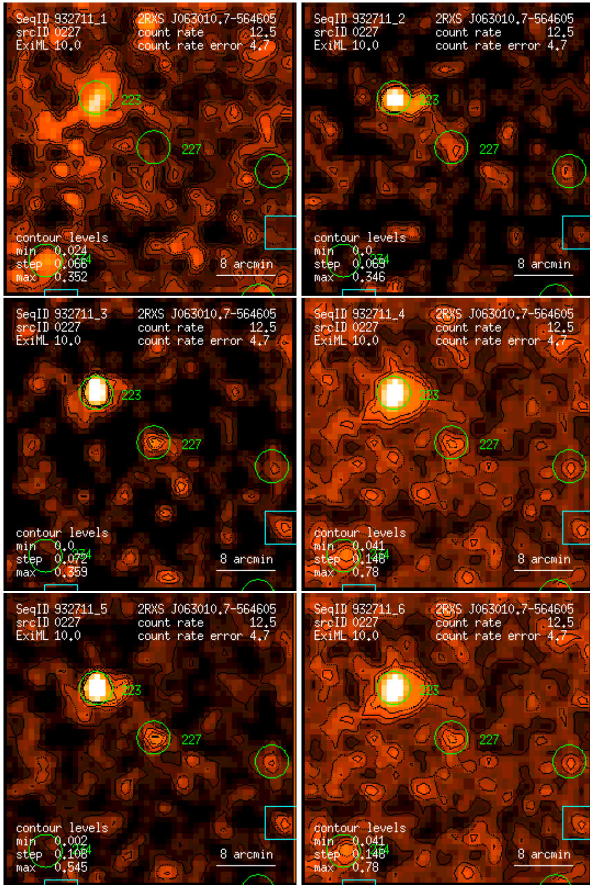
Figure 227: RASS 932711: detection 0227: band rate images, Gaussian filter: (1) PSPC channels 11 – 41, (2) 52 – 90, (3) 91 – 201, (4) 11 – 235, (5) 52 – 201, (6) 11 – 201. Broad band rates in counts/ks. Band rate contour levels in counts/ks/arcmin 2 .
