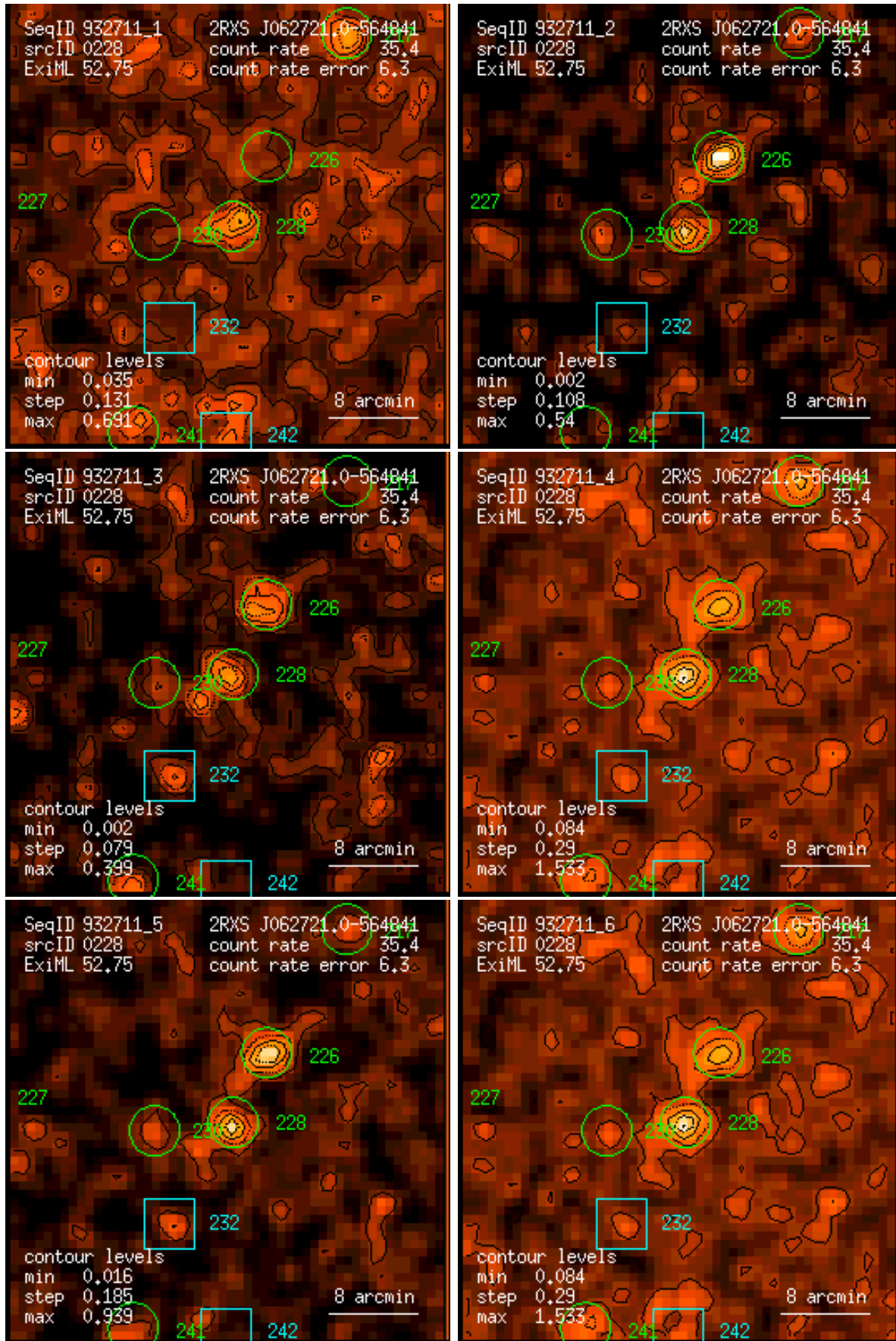
Figure 228: RASS 932711: detection 0228: band rate images, Gaussian filter: (1) PSPC channels 11 – 41, (2) 52 – 90, (3) 91 – 201, (4) 11 – 235, (5) 52 – 201, (6) 11 – 201. Broad band rates in counts/ks. Band rate contour levels in counts/ks/arcmin 2 .
