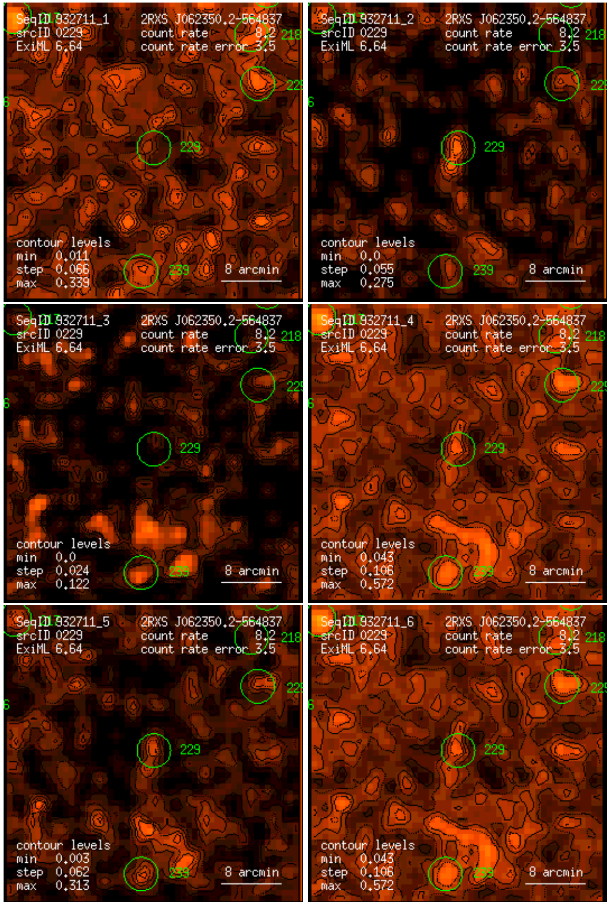
Figure 229: RASS 932711: detection 0229: band rate images, Gaussian filter: (1) PSPC channels 11 – 41, (2) 52 – 90, (3) 91 – 201, (4) 11 – 235, (5) 52 – 201, (6) 11 – 201. Broad band rates in counts/ks. Band rate contour levels in counts/ks/arcmin 2 .
