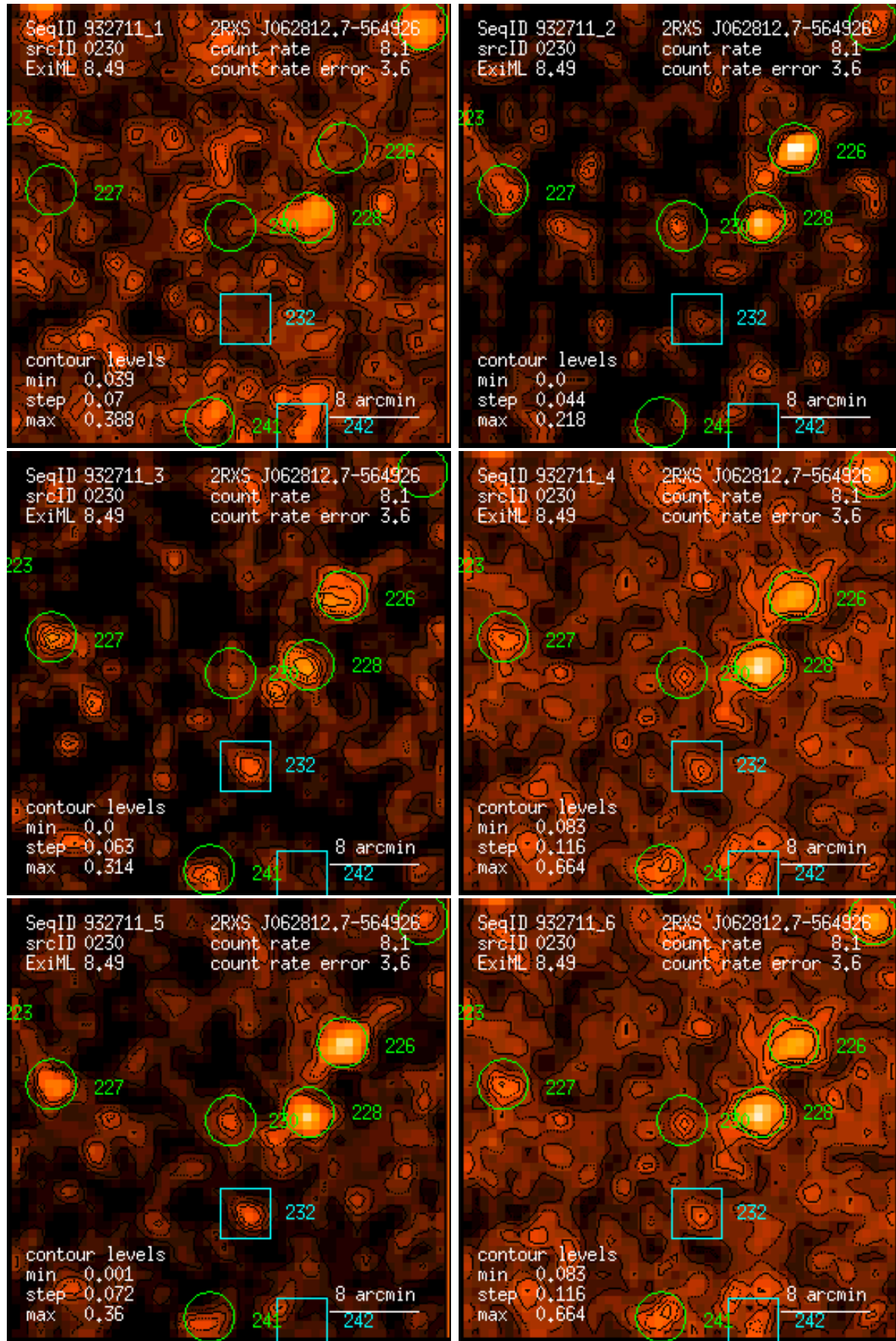
Figure 230: RASS 932711: detection 0230: band rate images, Gaussian filter: (1) PSPC channels 11 – 41, (2) 52 – 90, (3) 91 – 201, (4) 11 – 235, (5) 52 – 201, (6) 11 – 201. Broad band rates in counts/ks. Band rate contour levels in counts/ks/arcmin 2 .
