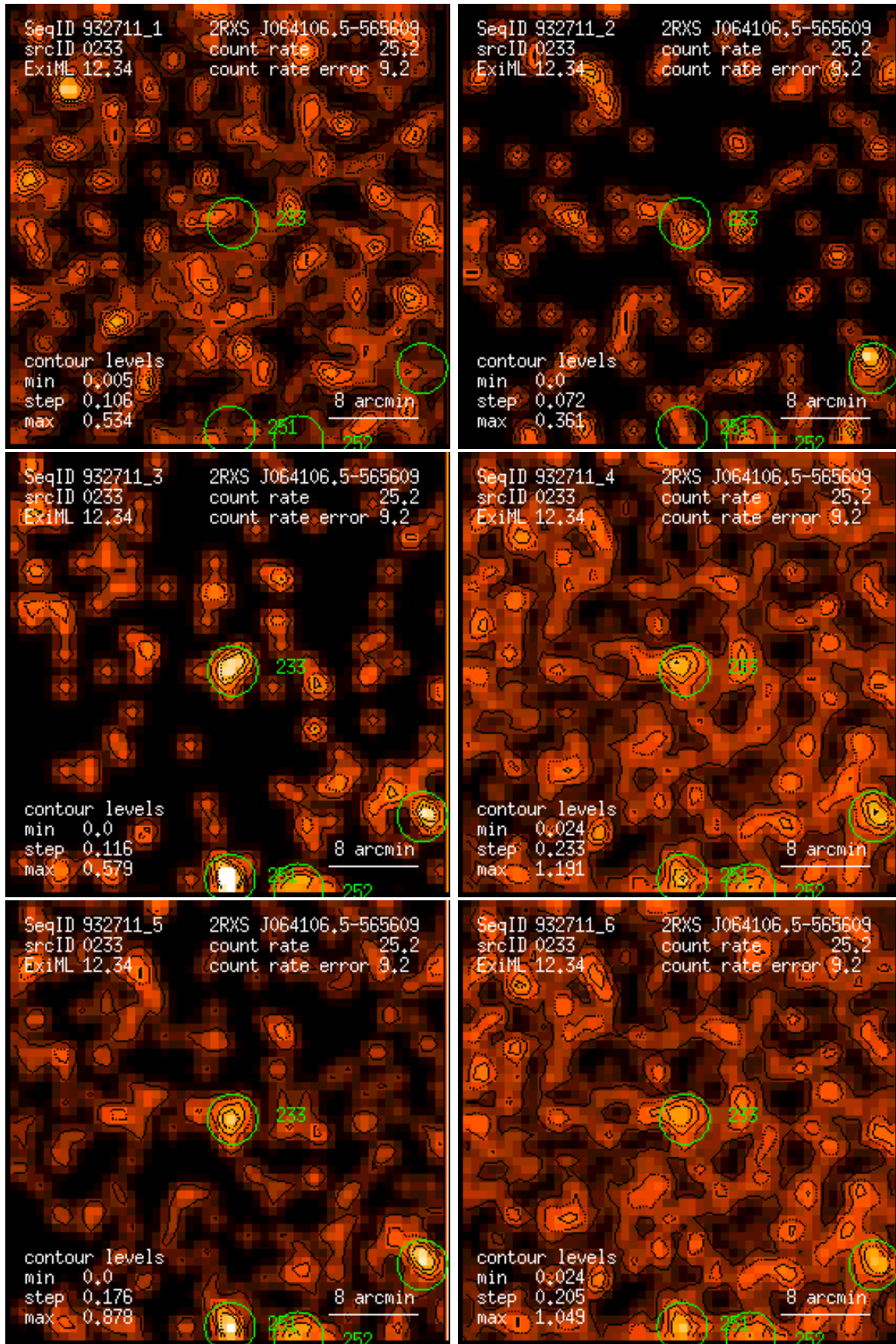
Figure 233: RASS 932711: detection 0233: band rate images, Gaussian filter: (1) PSPC channels 11 – 41, (2) 52 – 90, (3) 91 – 201, (4) 11 – 235, (5) 52 – 201, (6) 11 – 201. Broad band rates in counts/ks. Band rate contour levels in counts/ks/arcmin 2 .
