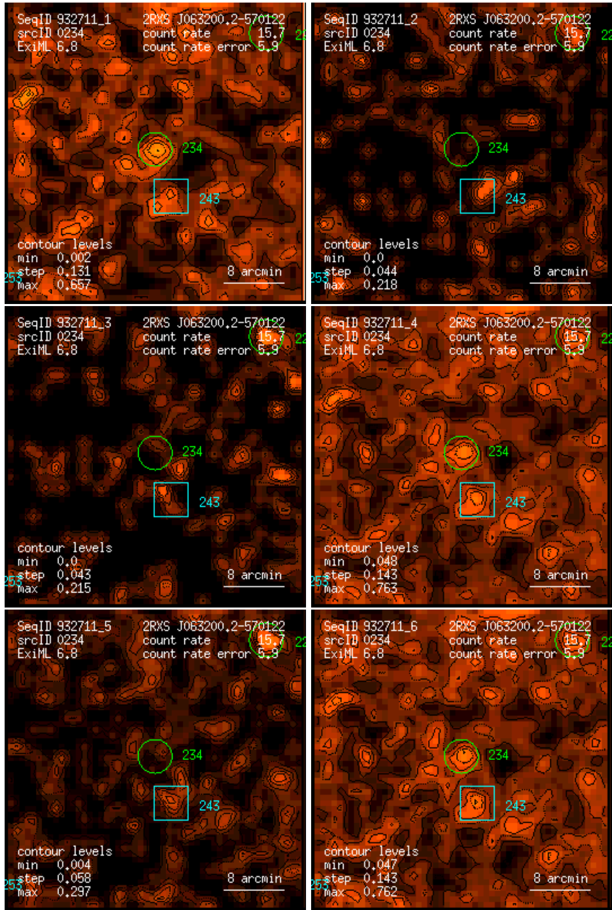
Figure 234: RASS 932711: detection 0234: band rate images, Gaussian filter: (1) PSPC channels 11 – 41, (2) 52 – 90, (3) 91 – 201, (4) 11 – 235, (5) 52 – 201, (6) 11 – 201. Broad band rates in counts/ks. Band rate contour levels in counts/ks/arcmin 2 .
