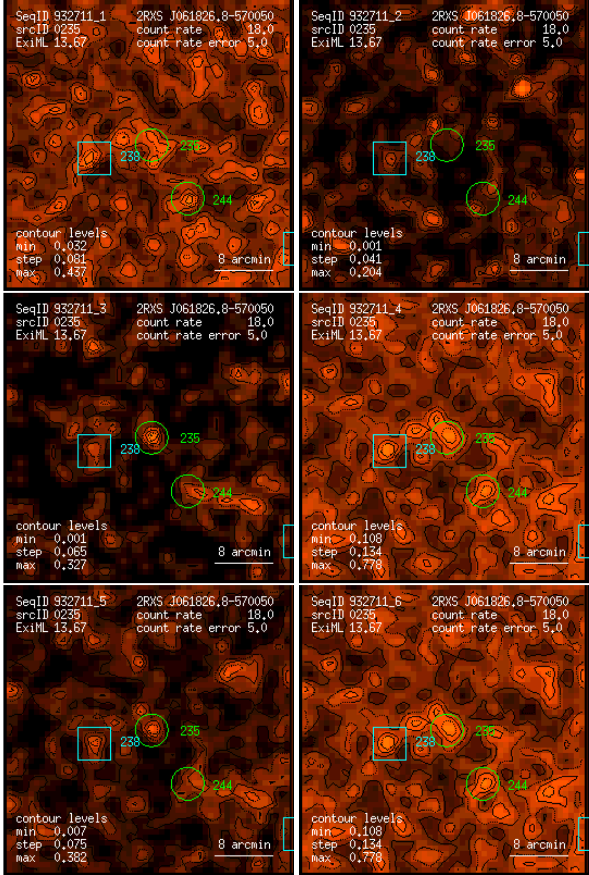
Figure 235: RASS 932711: detection 0235: band rate images, Gaussian filter: (1) PSPC channels 11 – 41, (2) 52 – 90, (3) 91 – 201, (4) 11 – 235, (5) 52 – 201, (6) 11 – 201. Broad band rates in counts/ks. Band rate contour levels in counts/ks/arcmin 2 .
