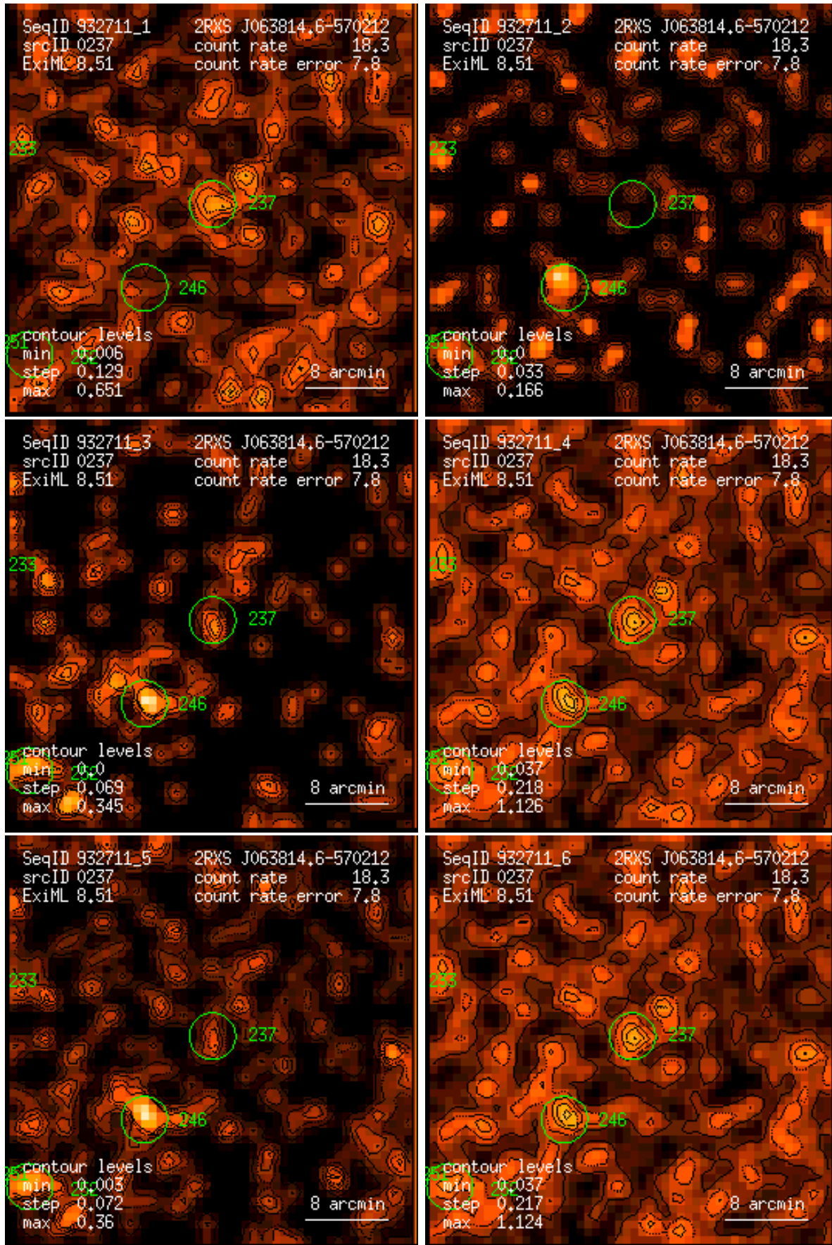
Figure 237: RASS 932711: detection 0237: band rate images, Gaussian filter: (1) PSPC channels 11 – 41, (2) 52 – 90, (3) 91 – 201, (4) 11 – 235, (5) 52 – 201, (6) 11 – 201. Broad band rates in counts/ks. Band rate contour levels in counts/ks/arcmin 2 .
