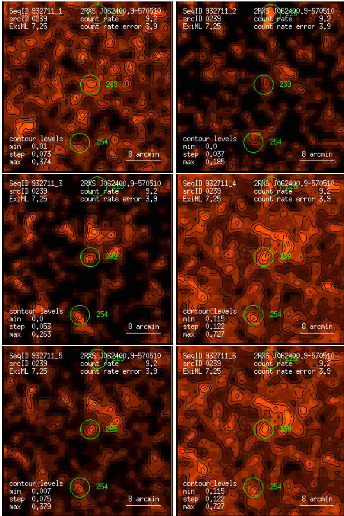
Figure 239: RASS 932711: detection 0239: band rate images, Gaussian filter: (1) PSPC channels 11 – 41, (2) 52 – 90, (3) 91 – 201, (4) 11 – 235, (5) 52 – 201, (6) 11 – 201. Broad band rates in counts/ks. Band rate contour levels in counts/ks/arcmin 2 .
