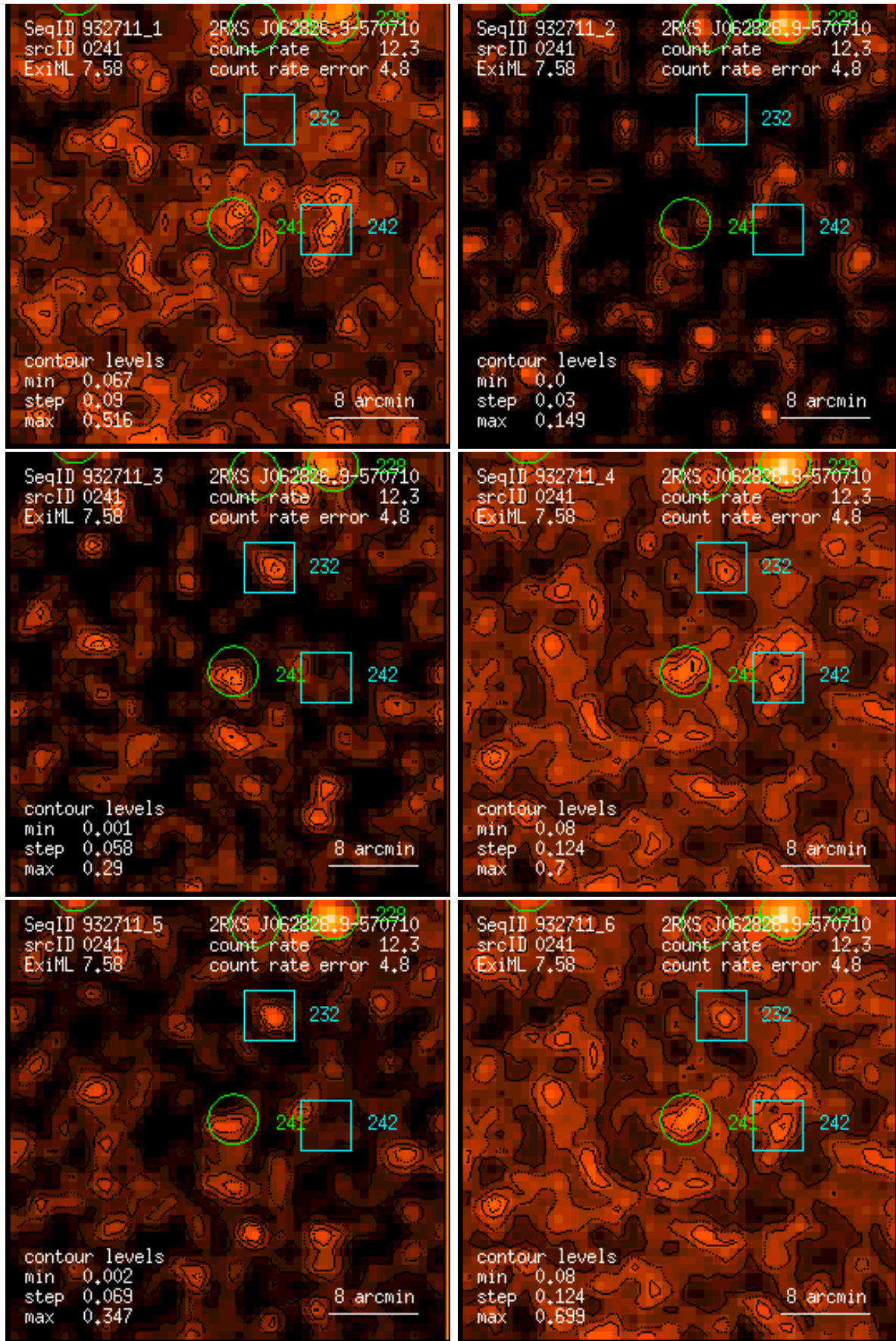
Figure 241: RASS 932711: detection 0241: band rate images, Gaussian filter: (1) PSPC channels 11 – 41, (2) 52 – 90, (3) 91 – 201, (4) 11 – 235, (5) 52 – 201, (6) 11 – 201. Broad band rates in counts/ks. Band rate contour levels in counts/ks/arcmin 2 .
