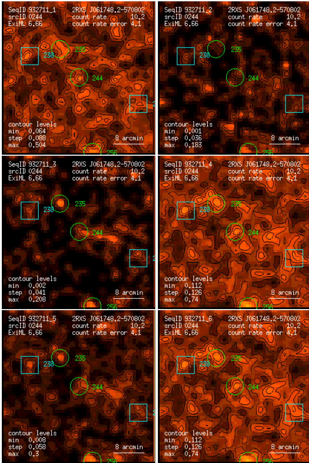
Figure 244: RASS 932711: detection 0244: band rate images, Gaussian filter: (1) PSPC channels 11 – 41, (2) 52 – 90, (3) 91 – 201, (4) 11 – 235, (5) 52 – 201, (6) 11 – 201. Broad band rates in counts/ks. Band rate contour levels in counts/ks/arcmin 2 .
