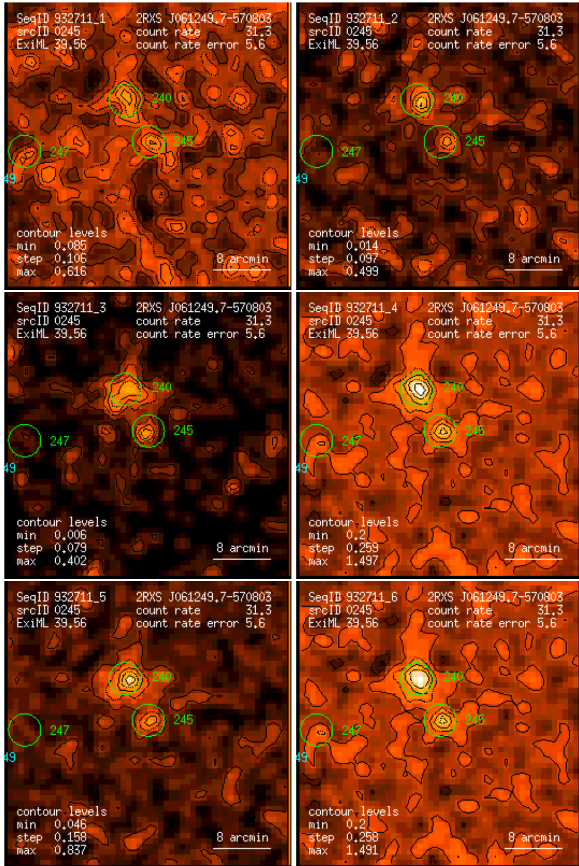
Figure 245: RASS 932711: detection 0245: band rate images, Gaussian filter: (1) PSPC channels 11 – 41, (2) 52 – 90, (3) 91 – 201, (4) 11 – 235, (5) 52 – 201, (6) 11 – 201. Broad band rates in counts/ks. Band rate contour levels in counts/ks/arcmin 2 .
