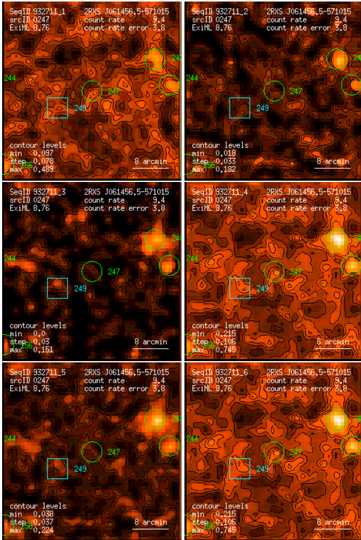
Figure 247: RASS 932711: detection 0247: band rate images, Gaussian filter: (1) PSPC channels 11 – 41, (2) 52 – 90, (3) 91 – 201, (4) 11 – 235, (5) 52 – 201, (6) 11 – 201. Broad band rates in counts/ks. Band rate contour levels in counts/ks/arcmin 2 .
