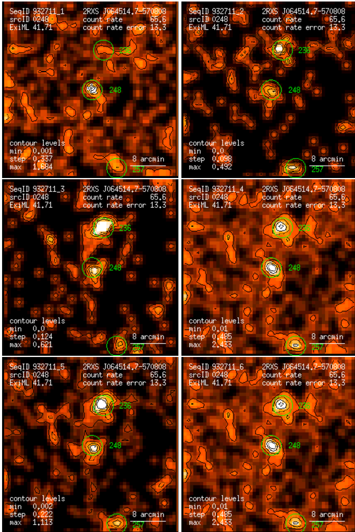
Figure 248: RASS 932711: detection 0248: band rate images, Gaussian filter: (1) PSPC channels 11 – 41, (2) 52 – 90, (3) 91 – 201, (4) 11 – 235, (5) 52 – 201, (6) 11 – 201. Broad band rates in counts/ks. Band rate contour levels in counts/ks/arcmin 2 .
