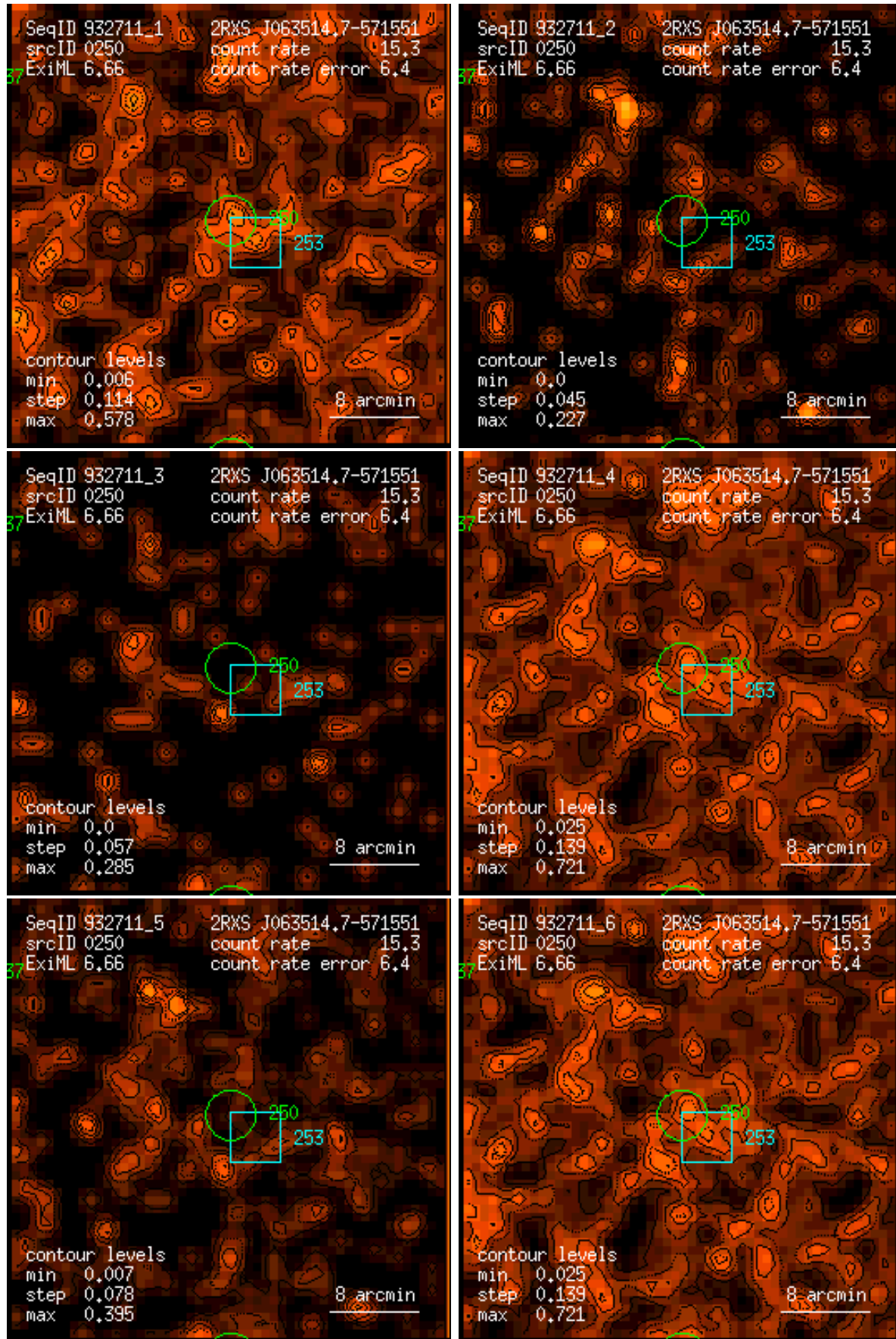
Figure 250: RASS 932711: detection 0250: band rate images, Gaussian filter: (1) PSPC channels 11 – 41, (2) 52 – 90, (3) 91 – 201, (4) 11 – 235, (5) 52 – 201, (6) 11 – 201. Broad band rates in counts/ks. Band rate contour levels in counts/ks/arcmin 2 .
