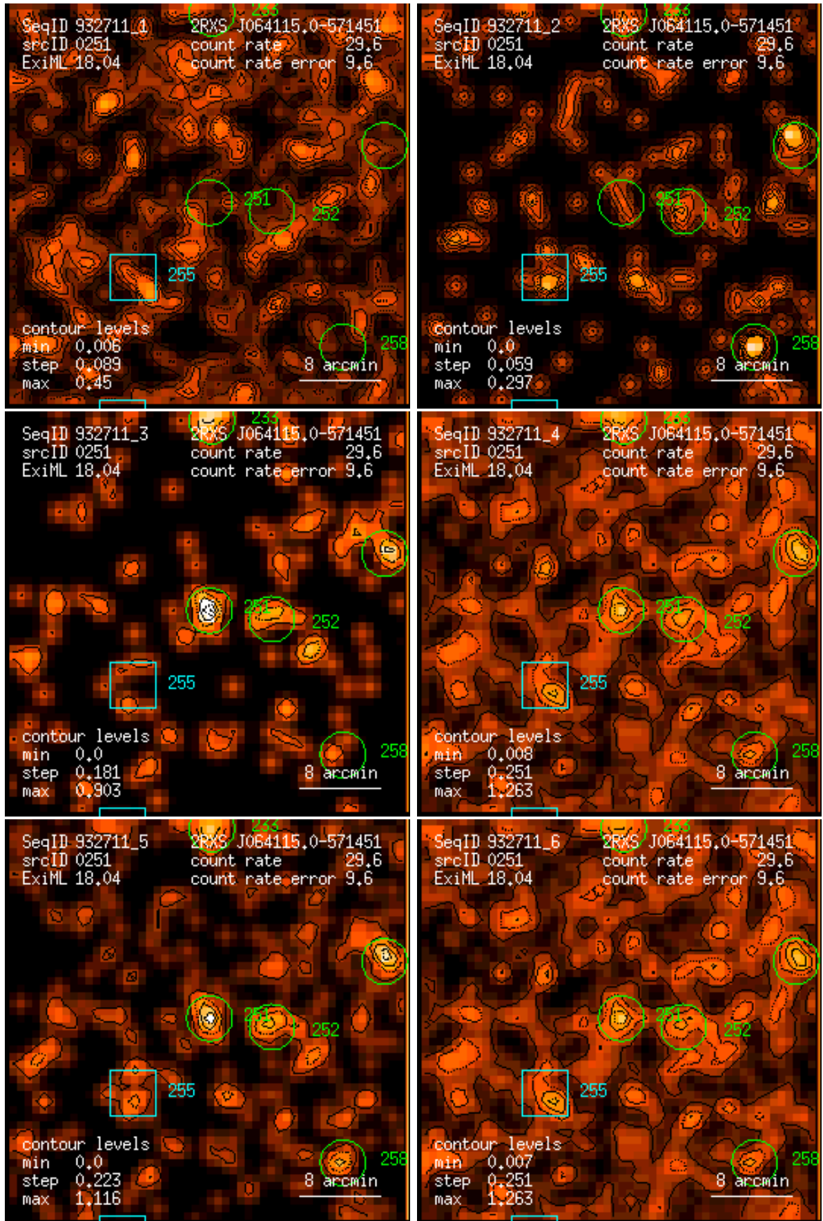
Figure 251: RASS 932711: detection 0251: band rate images, Gaussian filter: (1) PSPC channels 11 – 41, (2) 52 – 90, (3) 91 – 201, (4) 11 – 235, (5) 52 – 201, (6) 11 – 201. Broad band rates in counts/ks. Band rate contour levels in counts/ks/arcmin 2 .
