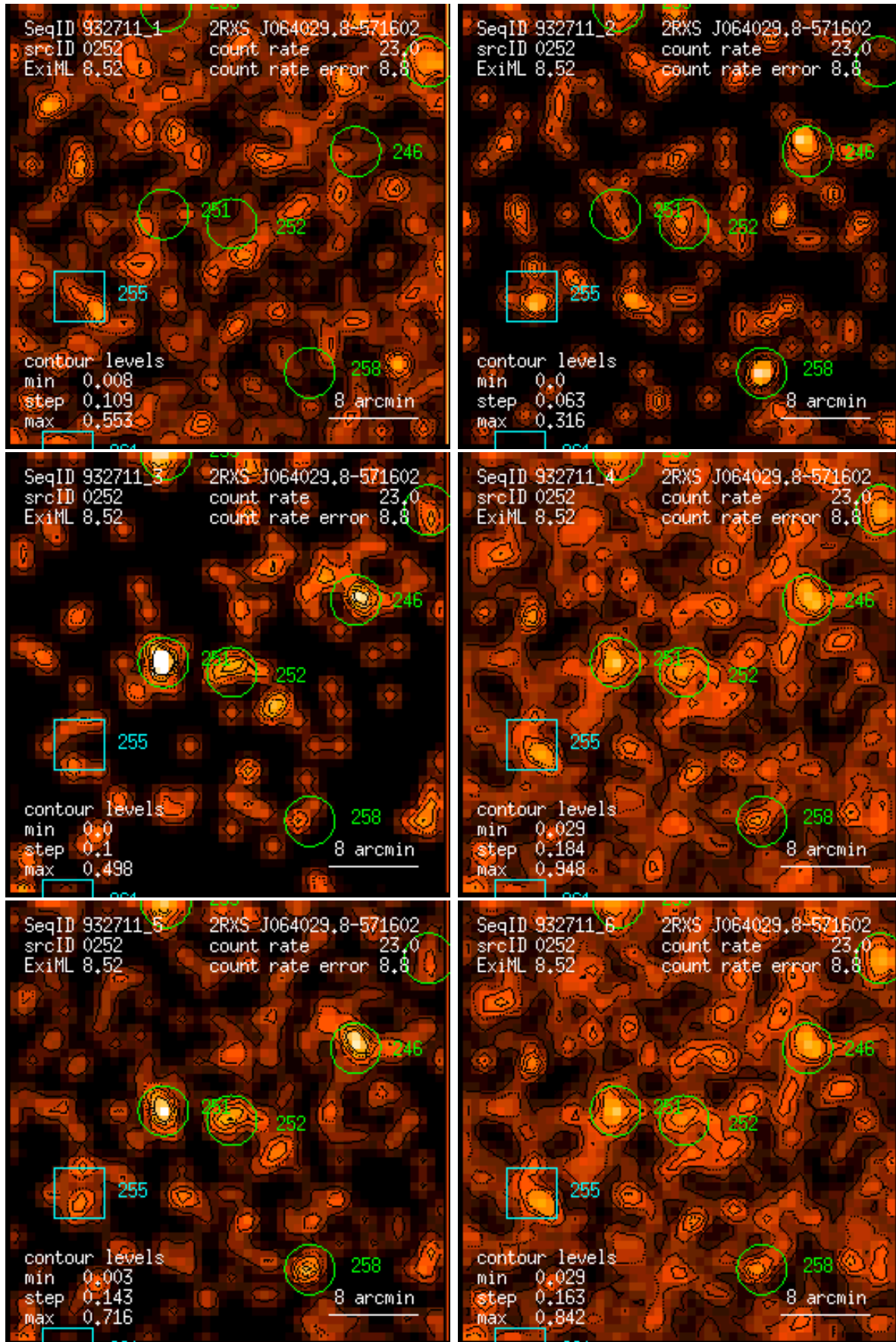
Figure 252: RASS 932711: detection 0252: band rate images, Gaussian filter: (1) PSPC channels 11 – 41, (2) 52 – 90, (3) 91 – 201, (4) 11 – 235, (5) 52 – 201, (6) 11 – 201. Broad band rates in counts/ks. Band rate contour levels in counts/ks/arcmin 2 .
