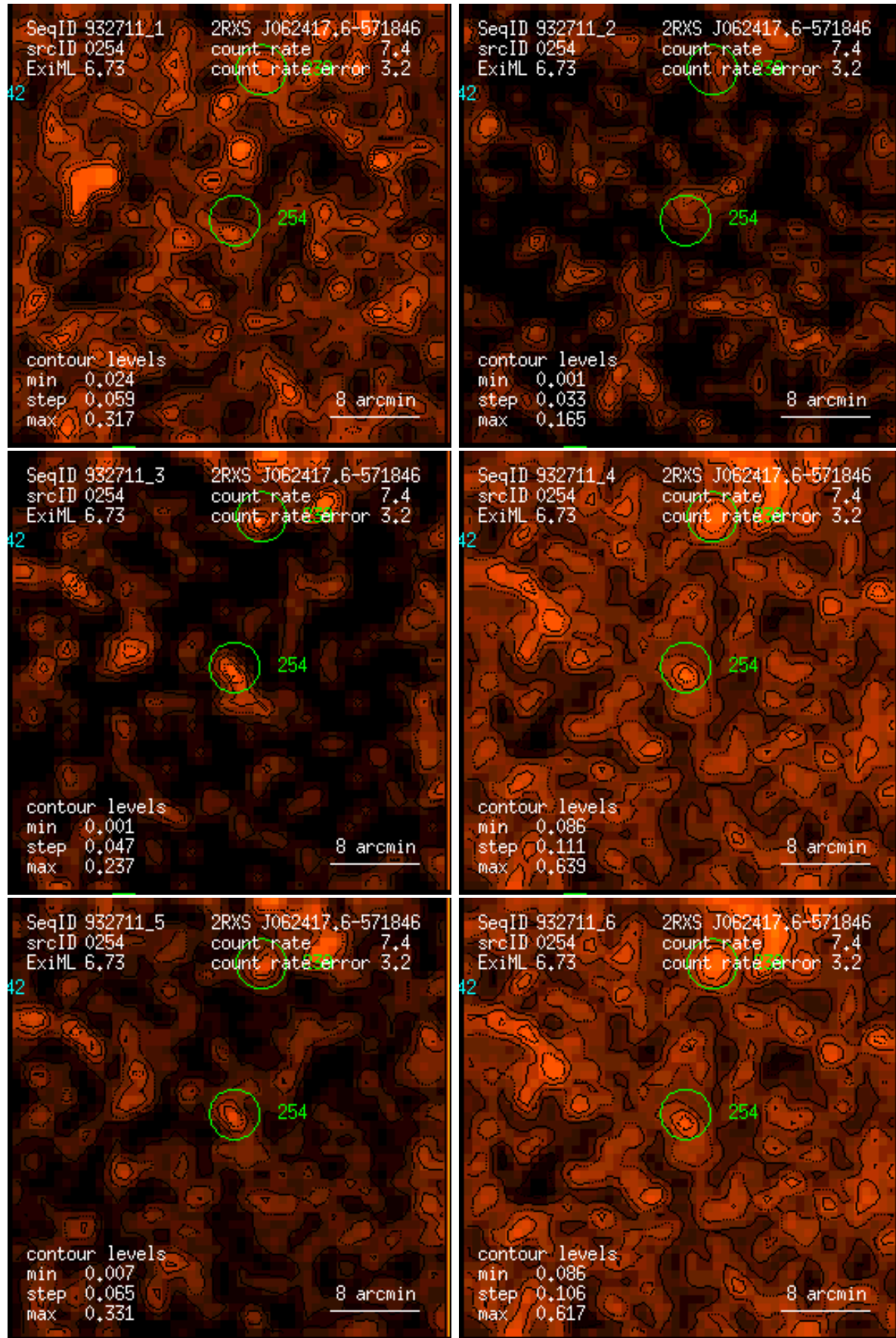
Figure 254: RASS 932711: detection 0254: band rate images, Gaussian filter: (1) PSPC channels 11 – 41, (2) 52 – 90, (3) 91 – 201, (4) 11 – 235, (5) 52 – 201, (6) 11 – 201. Broad band rates in counts/ks. Band rate contour levels in counts/ks/arcmin 2 .
