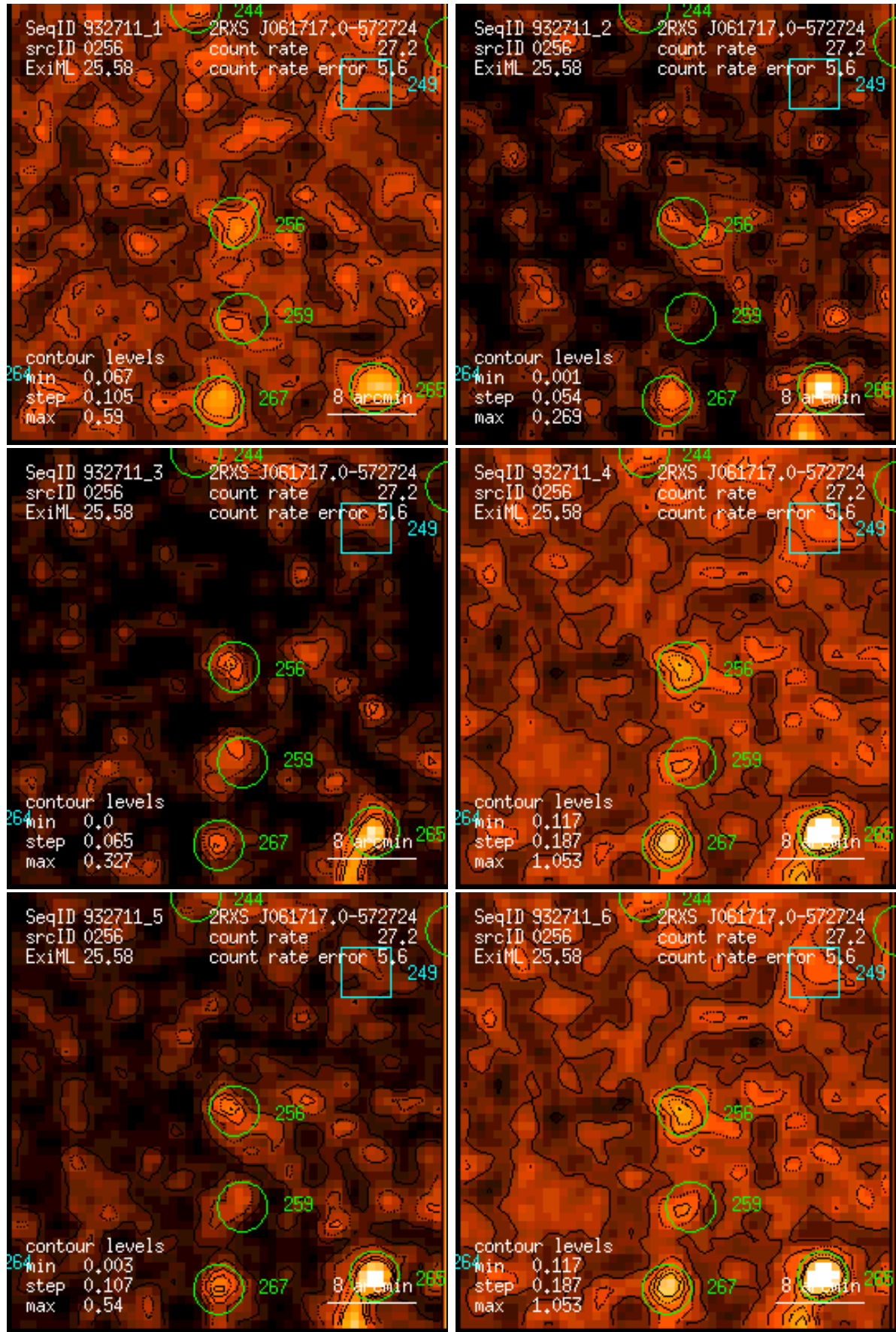
Figure 256: RASS 932711: detection 0256: band rate images, Gaussian filter: (1) PSPC channels 11 – 41, (2) 52 – 90, (3) 91 – 201, (4) 11 – 235, (5) 52 – 201, (6) 11 – 201. Broad band rates in counts/ks. Band rate contour levels in counts/ks/arcmin 2 .
