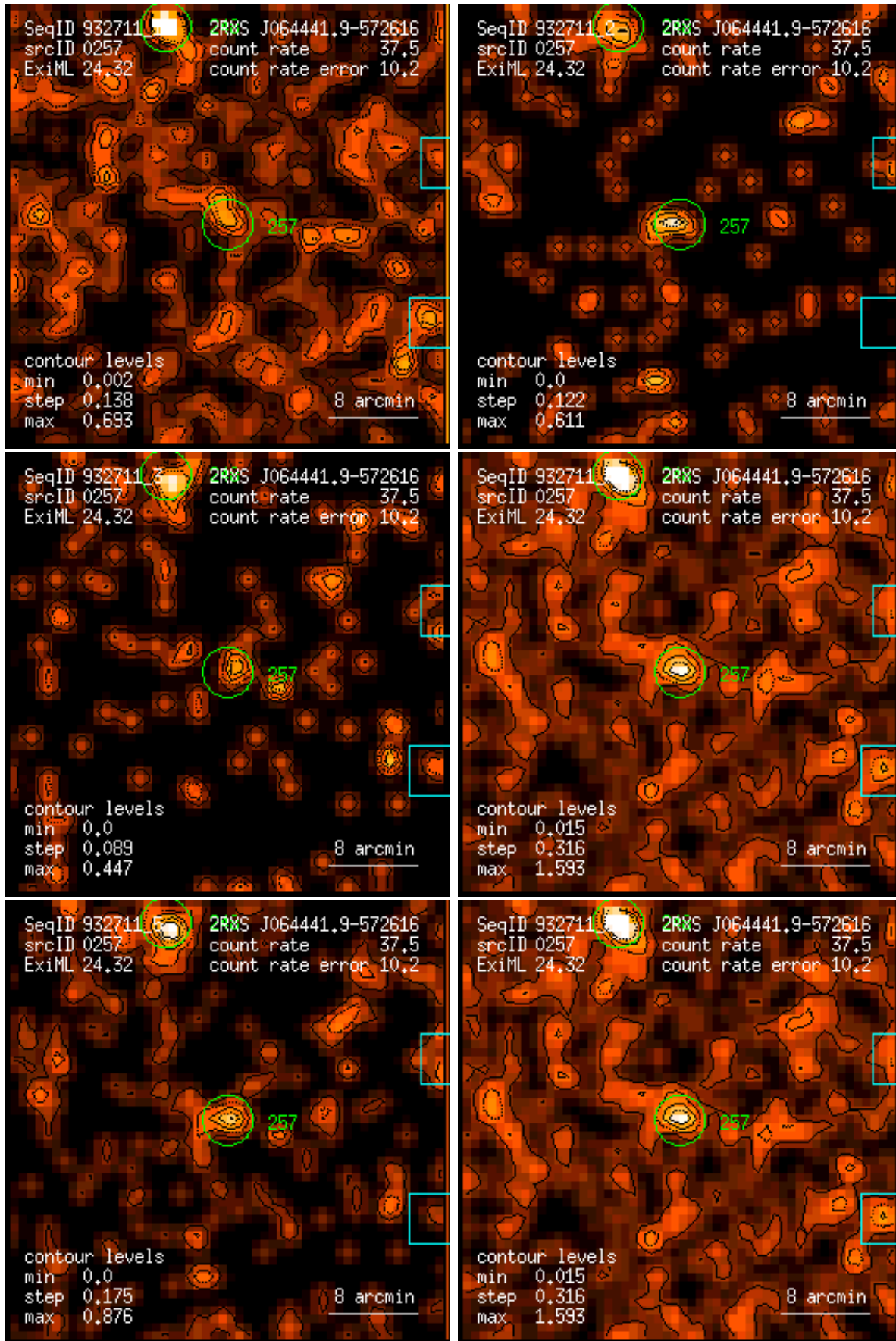
Figure 257: RASS 932711: detection 0257: band rate images, Gaussian filter: (1) PSPC channels 11 – 41, (2) 52 – 90, (3) 91 – 201, (4) 11 – 235, (5) 52 – 201, (6) 11 – 201. Broad band rates in counts/ks. Band rate contour levels in counts/ks/arcmin 2 .
