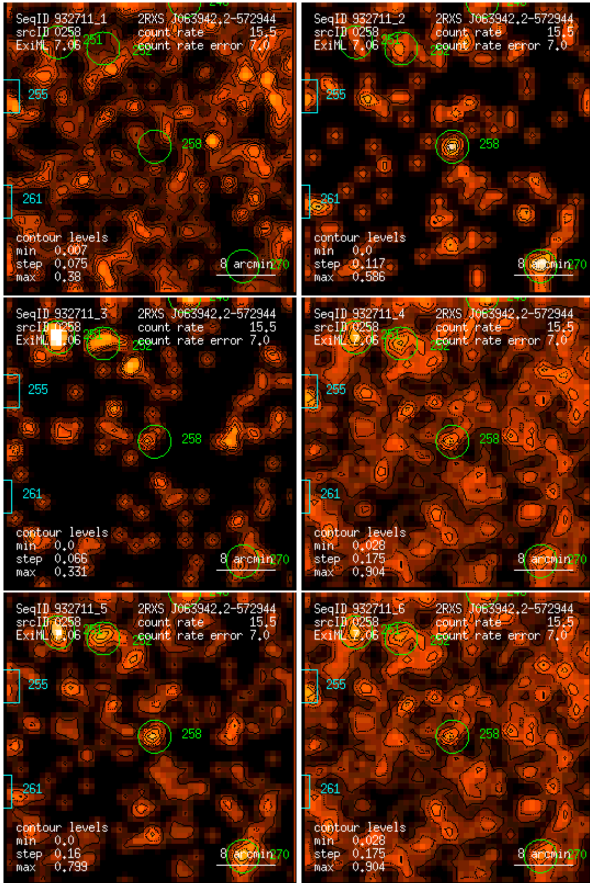
Figure 258: RASS 932711: detection 0258: band rate images, Gaussian filter: (1) PSPC channels 11 – 41, (2) 52 – 90, (3) 91 – 201, (4) 11 – 235, (5) 52 – 201, (6) 11 – 201. Broad band rates in counts/ks. Band rate contour levels in counts/ks/arcmin 2 .
