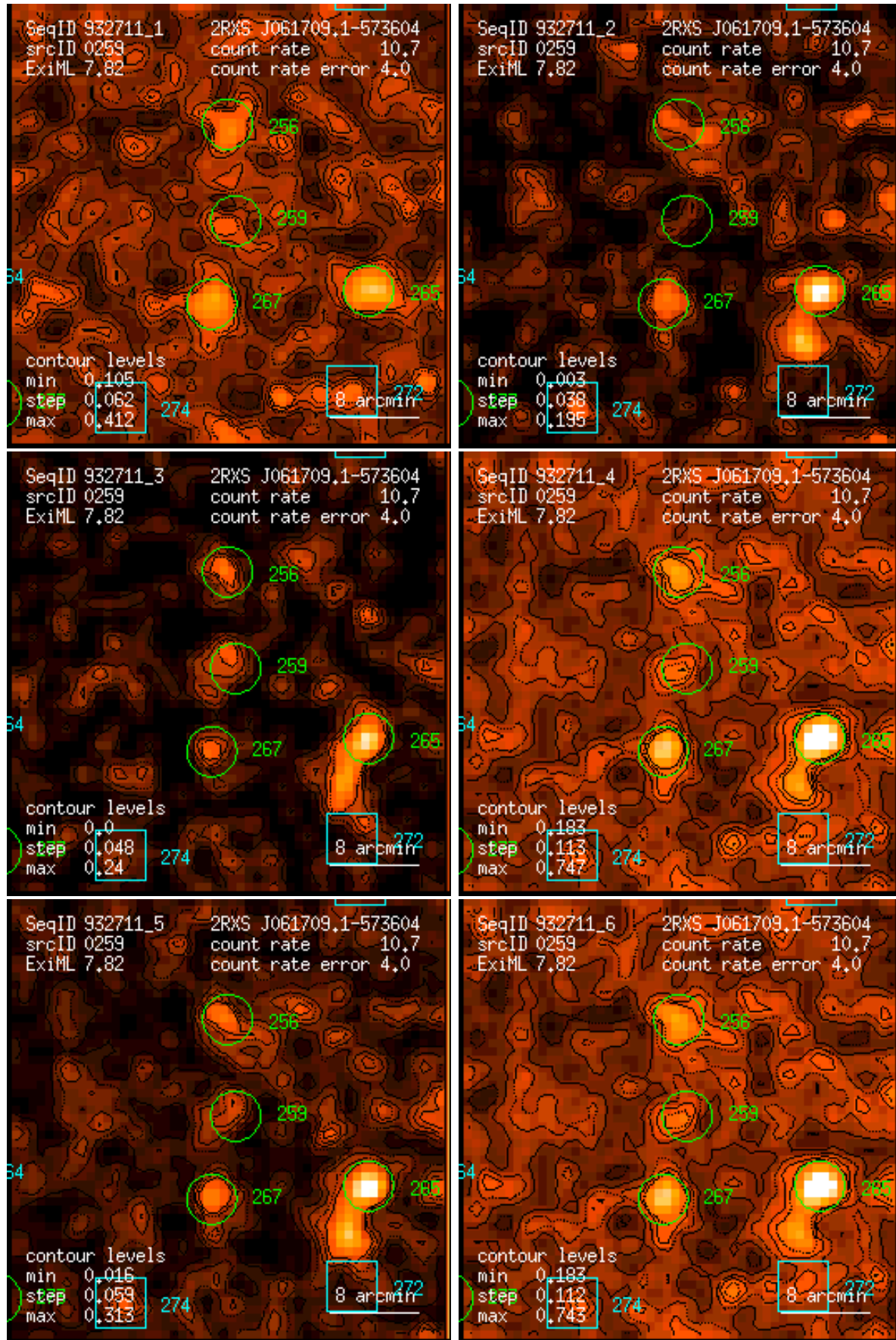
Figure 259: RASS 932711: detection 0259: band rate images, Gaussian filter: (1) PSPC channels 11 – 41, (2) 52 – 90, (3) 91 – 201, (4) 11 – 235, (5) 52 – 201, (6) 11 – 201. Broad band rates in counts/ks. Band rate contour levels in counts/ks/arcmin 2 .
