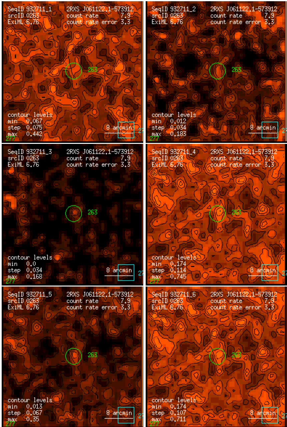
Figure 263: RASS 932711: detection 0263: band rate images, Gaussian filter: (1) PSPC channels 11 – 41, (2) 52 – 90, (3) 91 – 201, (4) 11 – 235, (5) 52 – 201, (6) 11 – 201. Broad band rates in counts/ks. Band rate contour levels in counts/ks/arcmin 2 .
