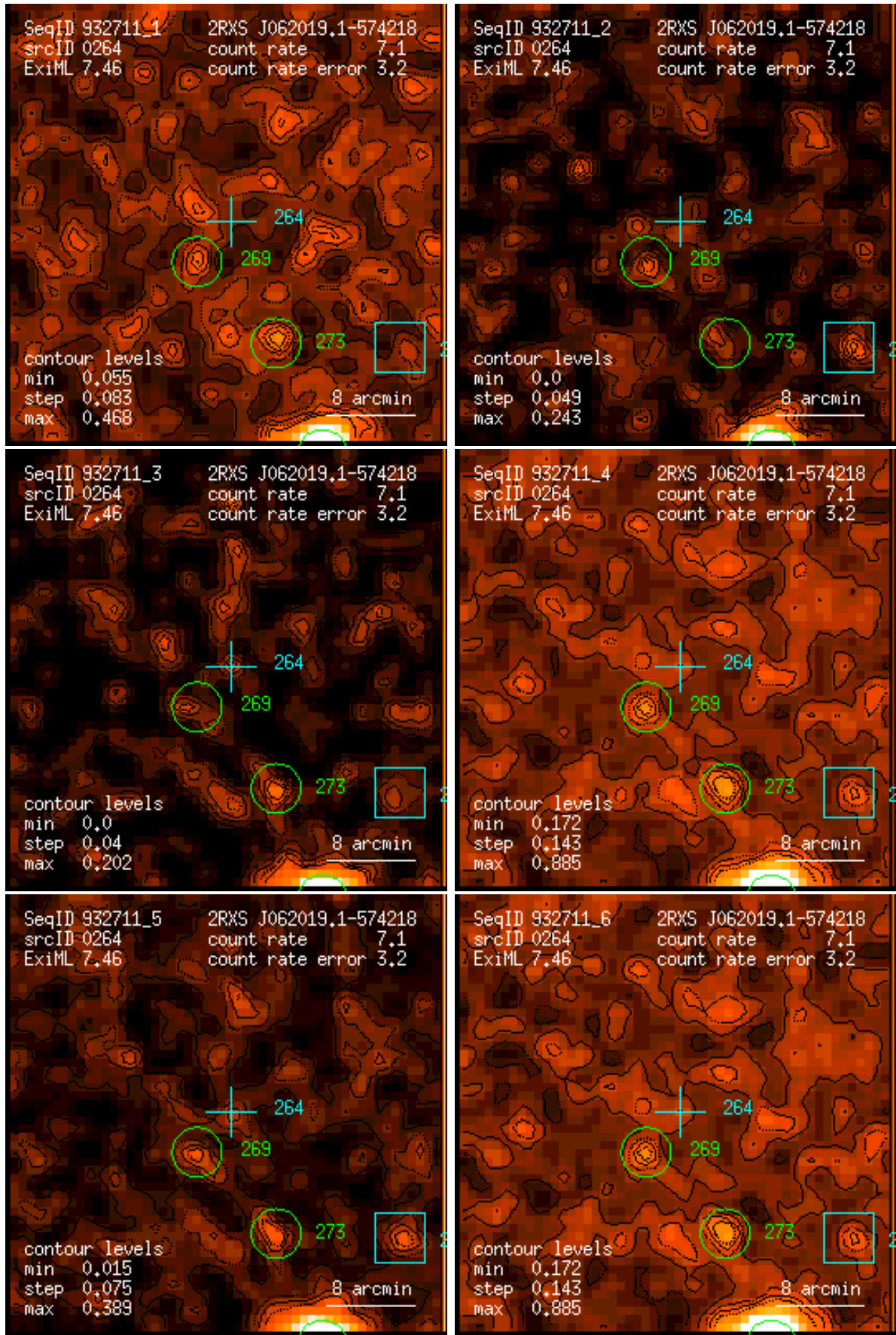
Figure 264: RASS 932711: detection 0264: band rate images, Gaussian filter: (1) PSPC channels 11 – 41, (2) 52 – 90, (3) 91 – 201, (4) 11 – 235, (5) 52 – 201, (6) 11 – 201. Broad band rates in counts/ks. Band rate contour levels in counts/ks/arcmin 2 .
