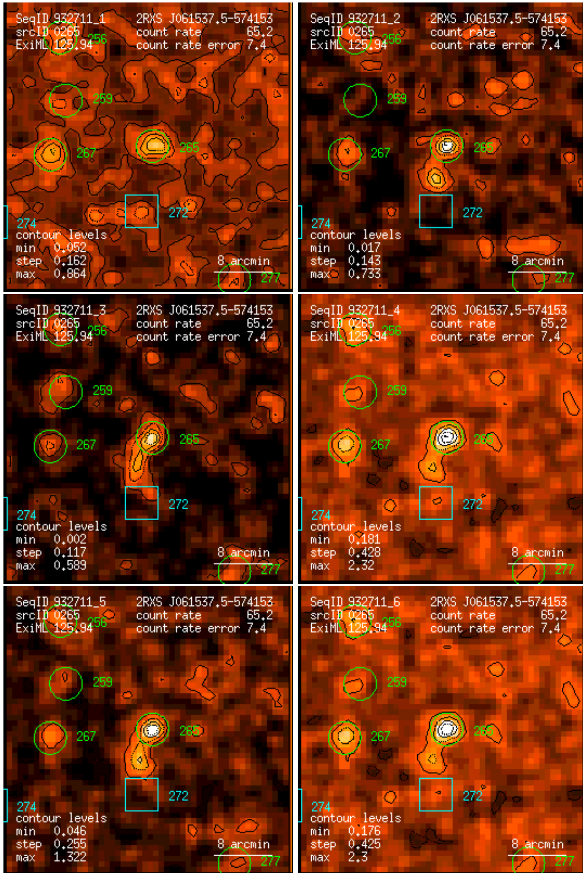
Figure 265: RASS 932711: detection 0265: band rate images, Gaussian filter: (1) PSPC channels 11 – 41, (2) 52 – 90, (3) 91 – 201, (4) 11 – 235, (5) 52 – 201, (6) 11 – 201. Broad band rates in counts/ks. Band rate contour levels in counts/ks/arcmin 2 .
