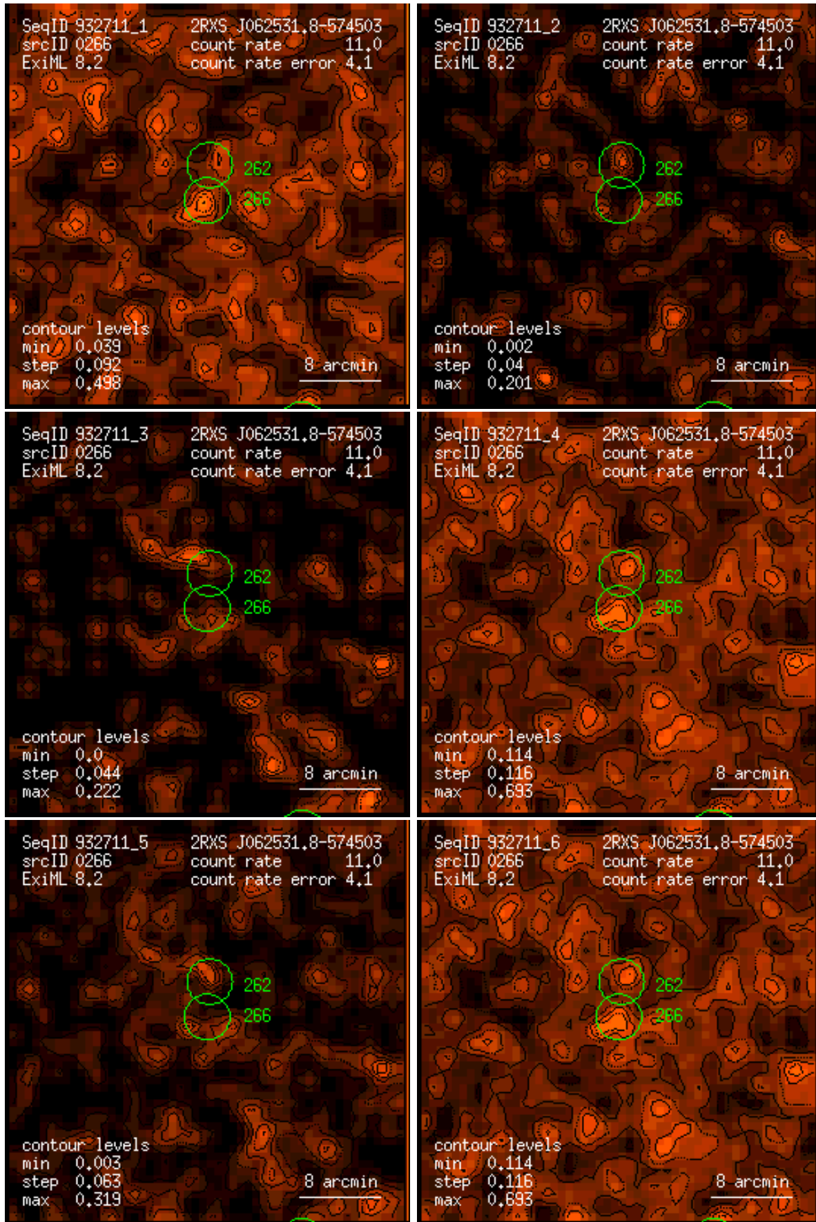
Figure 266: RASS 932711: detection 0266: band rate images, Gaussian filter: (1) PSPC channels 11 – 41, (2) 52 – 90, (3) 91 – 201, (4) 11 – 235, (5) 52 – 201, (6) 11 – 201. Broad band rates in counts/ks. Band rate contour levels in counts/ks/arcmin 2 .
