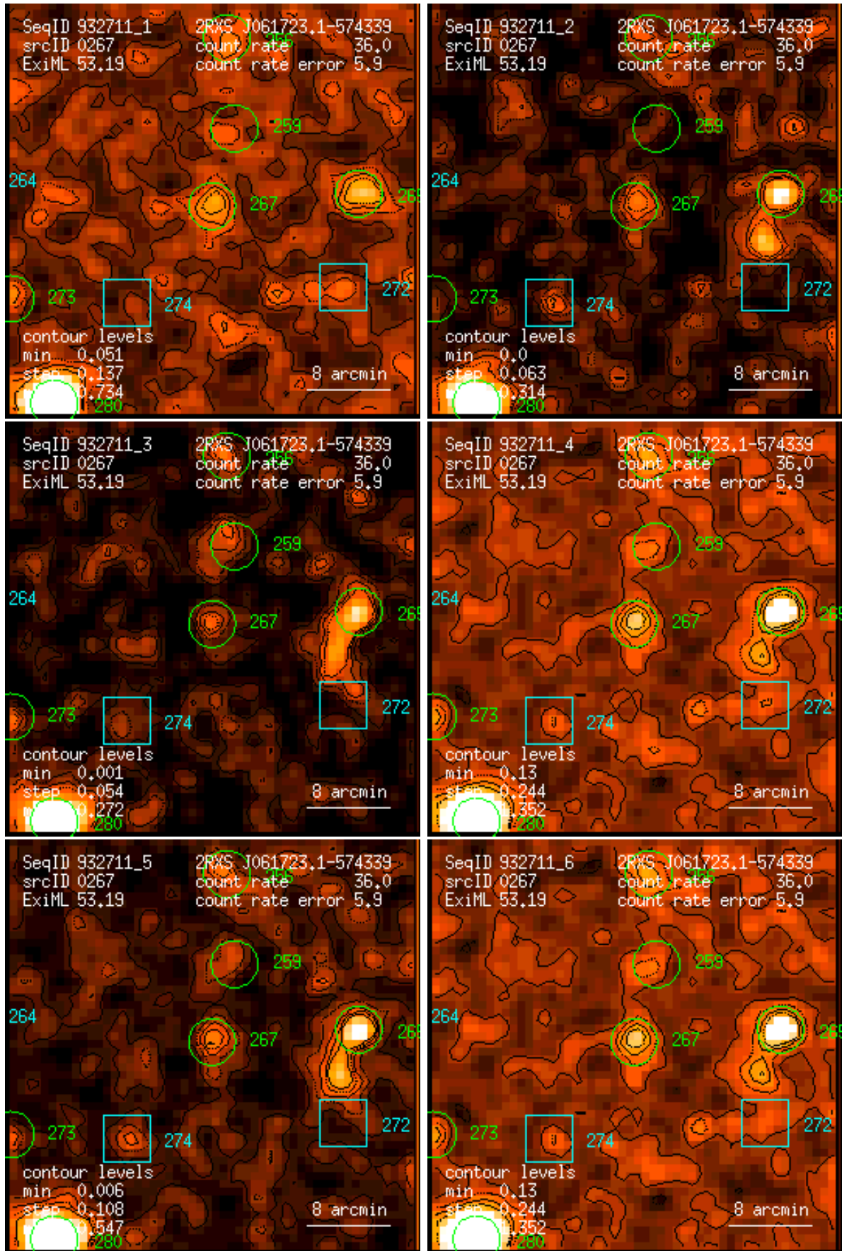
Figure 267: RASS 932711: detection 0267: band rate images, Gaussian filter: (1) PSPC channels 11 – 41, (2) 52 – 90, (3) 91 – 201, (4) 11 – 235, (5) 52 – 201, (6) 11 – 201. Broad band rates in counts/ks. Band rate contour levels in counts/ks/arcmin 2 .
