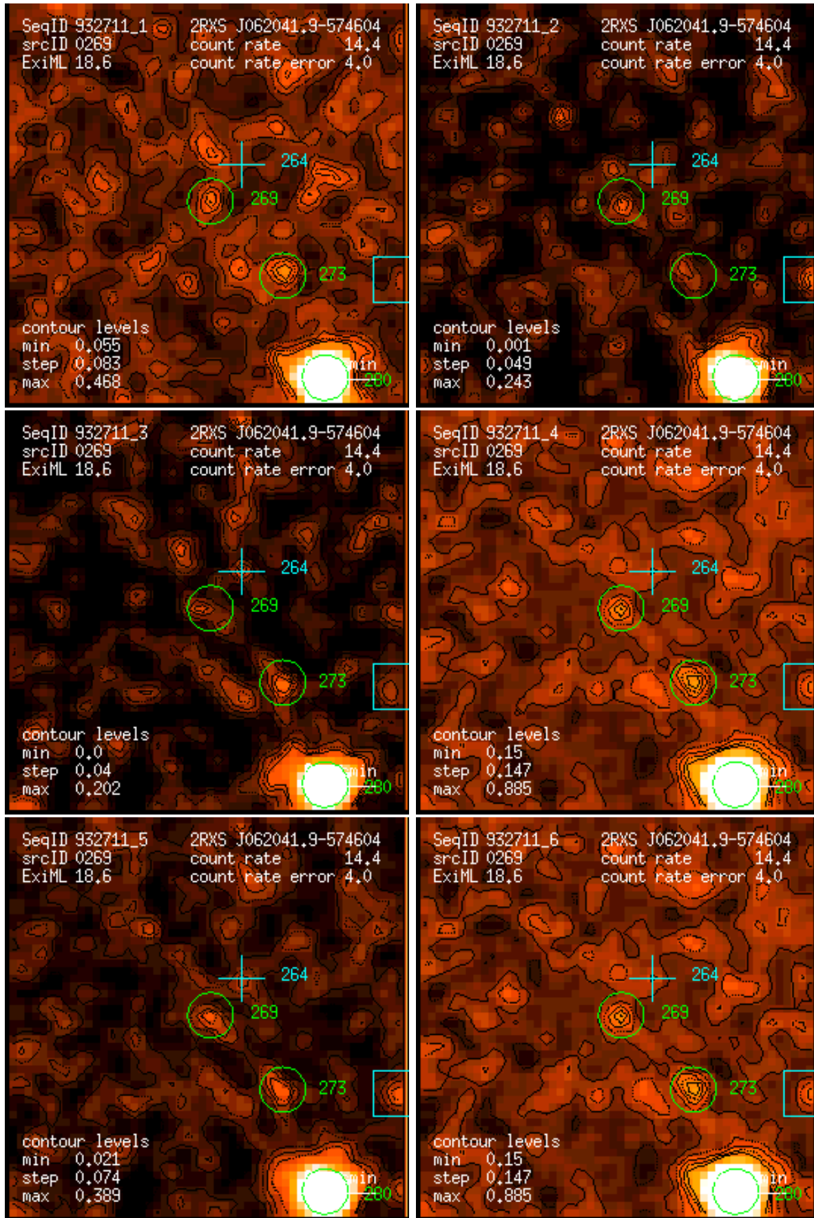
Figure 269: RASS 932711: detection 0269: band rate images, Gaussian filter: (1) PSPC channels 11 – 41, (2) 52 – 90, (3) 91 – 201, (4) 11 – 235, (5) 52 – 201, (6) 11 – 201. Broad band rates in counts/ks. Band rate contour levels in counts/ks/arcmin 2 .
