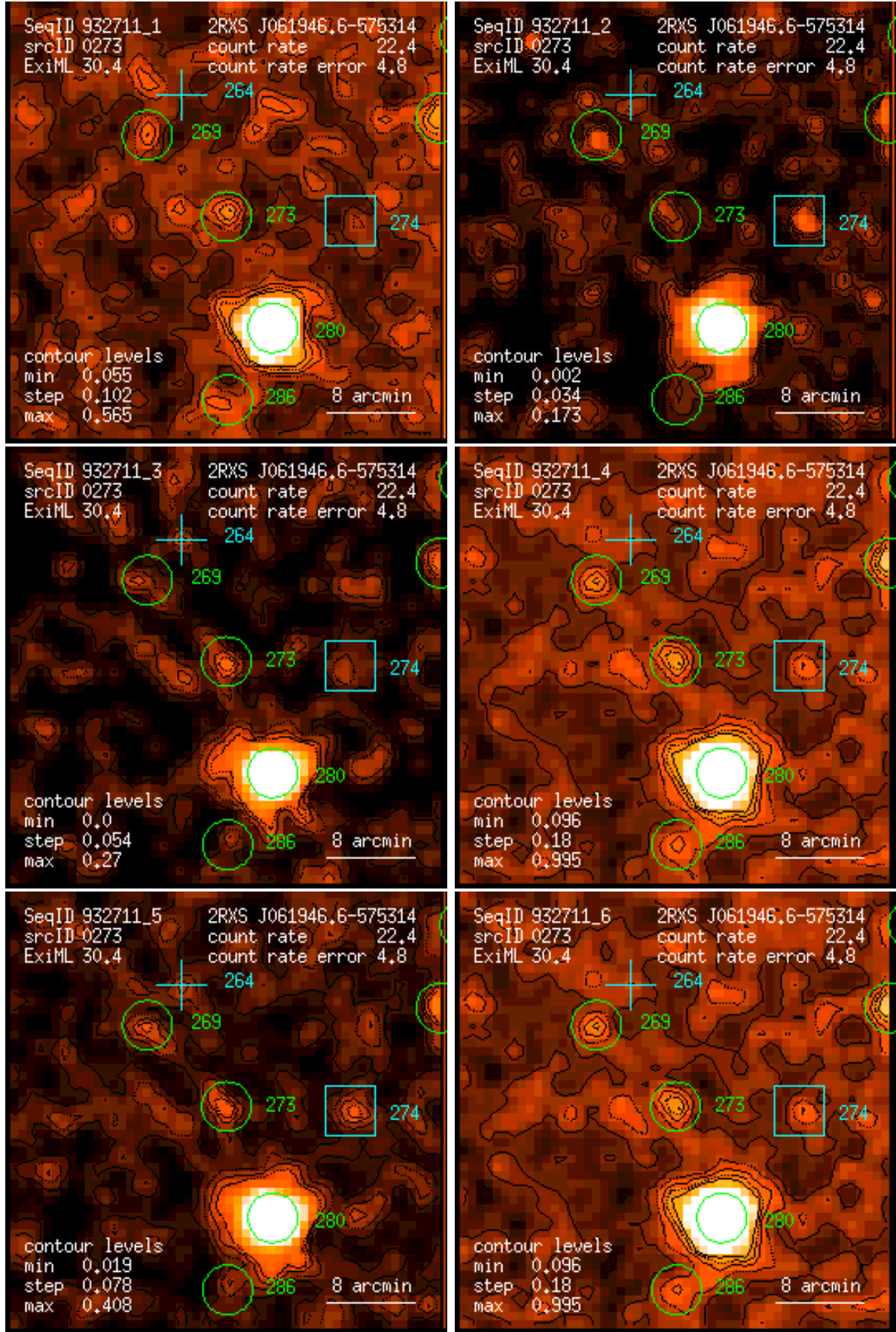
Figure 273: RASS 932711: detection 0273: band rate images, Gaussian filter: (1) PSPC channels 11 – 41, (2) 52 – 90, (3) 91 – 201, (4) 11 – 235, (5) 52 – 201, (6) 11 – 201. Broad band rates in counts/ks. Band rate contour levels in counts/ks/arcmin 2 .
