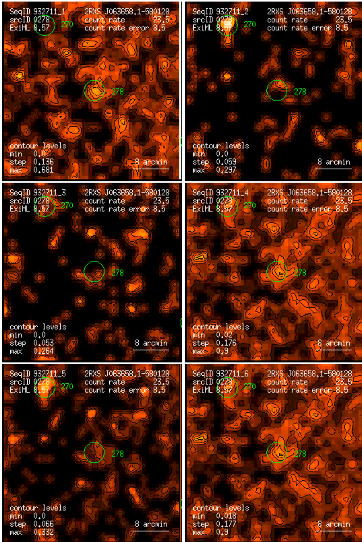
Figure 278: RASS 932711: detection 0278: band rate images, Gaussian filter: (1) PSPC channels 11 – 41, (2) 52 – 90, (3) 91 – 201, (4) 11 – 235, (5) 52 – 201, (6) 11 – 201. Broad band rates in counts/ks. Band rate contour levels in counts/ks/arcmin 2 .
