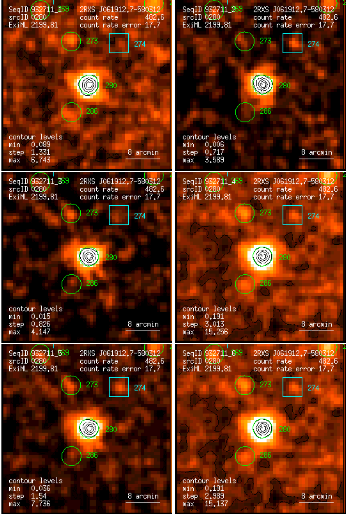
Figure 280: RASS 932711: detection 0280: band rate images, Gaussian filter: (1) PSPC channels 11 – 41, (2) 52 – 90, (3) 91 – 201, (4) 11 – 235, (5) 52 – 201, (6) 11 – 201. Broad band rates in counts/ks. Band rate contour levels in counts/ks/arcmin 2 .
