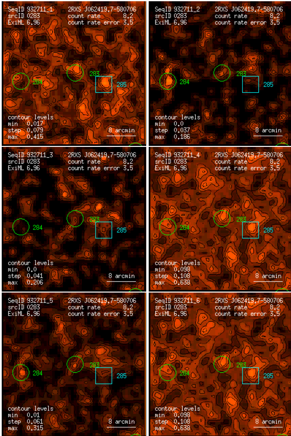
Figure 283: RASS 932711: detection 0283: band rate images, Gaussian filter: (1) PSPC channels 11 – 41, (2) 52 – 90, (3) 91 – 201, (4) 11 – 235, (5) 52 – 201, (6) 11 – 201. Broad band rates in counts/ks. Band rate contour levels in counts/ks/arcmin 2 .
