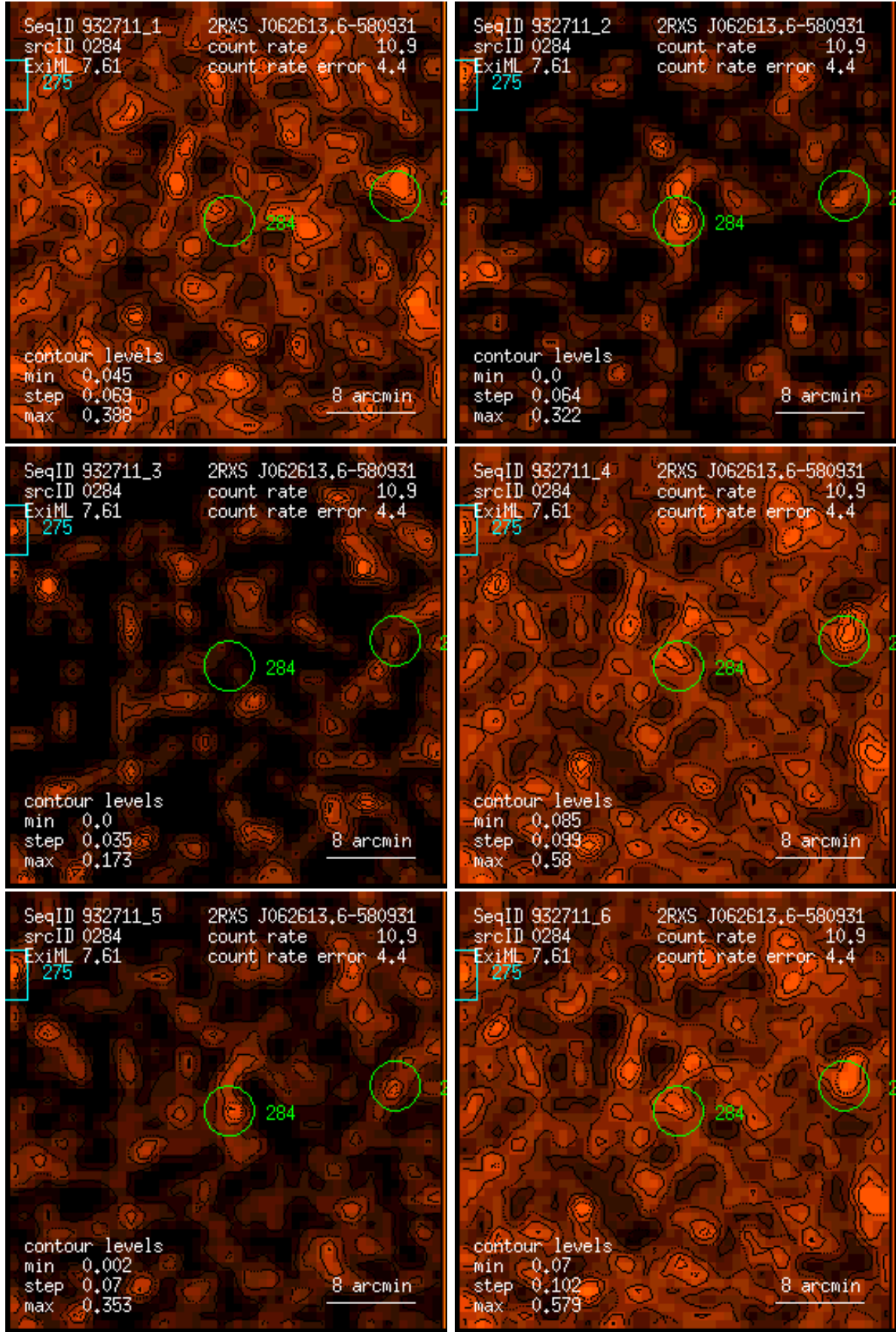
Figure 284: RASS 932711: detection 0284: band rate images, Gaussian filter: (1) PSPC channels 11 – 41, (2) 52 – 90, (3) 91 – 201, (4) 11 – 235, (5) 52 – 201, (6) 11 – 201. Broad band rates in counts/ks. Band rate contour levels in counts/ks/arcmin 2 .
