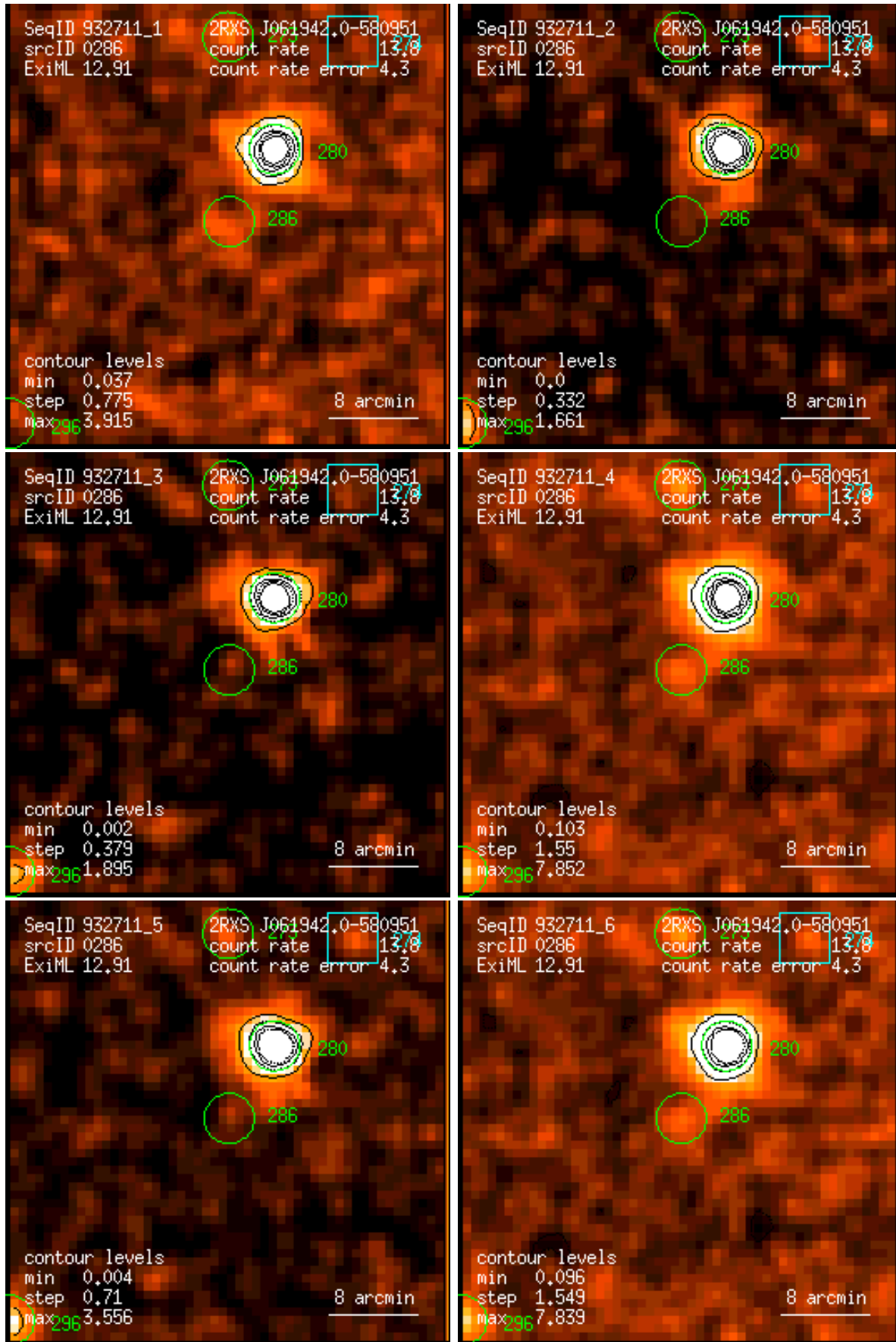
Figure 286: RASS 932711: detection 0286: band rate images, Gaussian filter: (1) PSPC channels 11 – 41, (2) 52 – 90, (3) 91 – 201, (4) 11 – 235, (5) 52 – 201, (6) 11 – 201. Broad band rates in counts/ks. Band rate contour levels in counts/ks/arcmin 2 .
