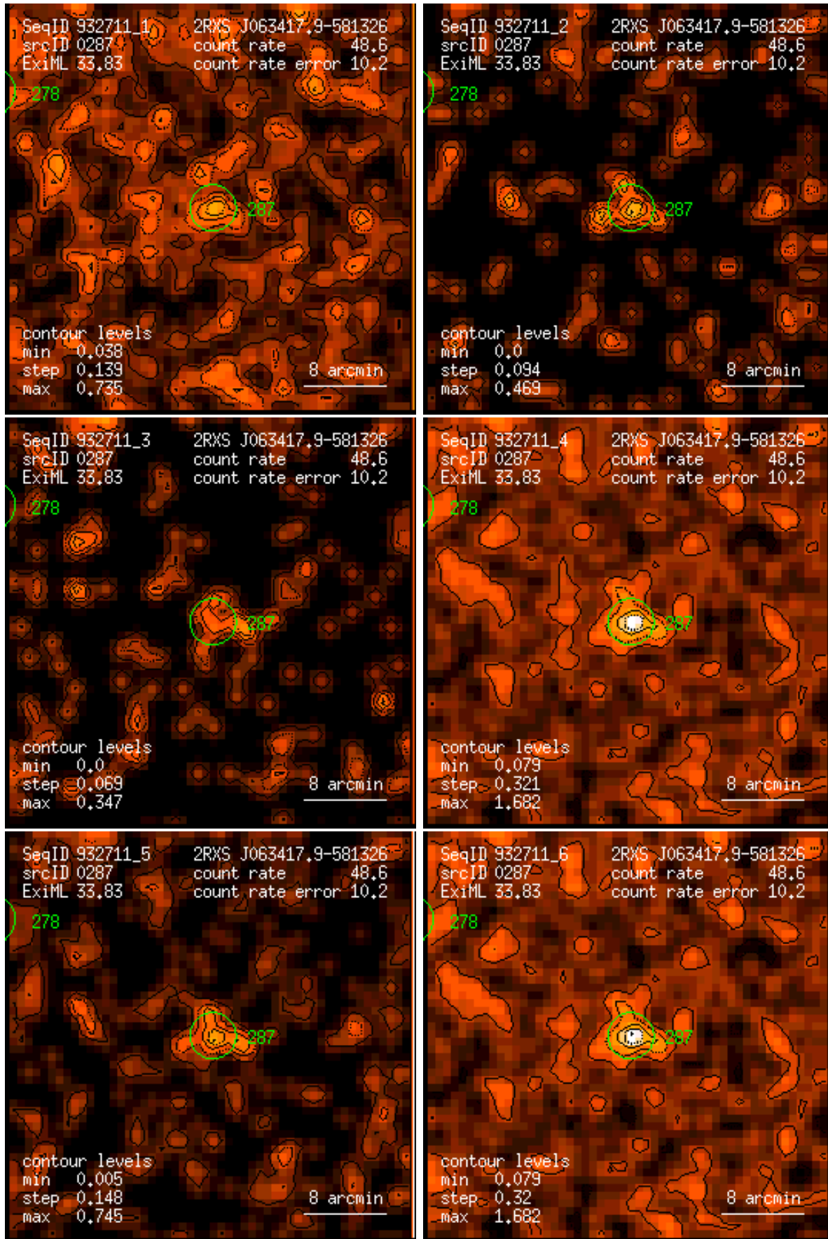
Figure 287: RASS 932711: detection 0287: band rate images, Gaussian filter: (1) PSPC channels 11 – 41, (2) 52 – 90, (3) 91 – 201, (4) 11 – 235, (5) 52 – 201, (6) 11 – 201. Broad band rates in counts/ks. Band rate contour levels in counts/ks/arcmin 2 .
