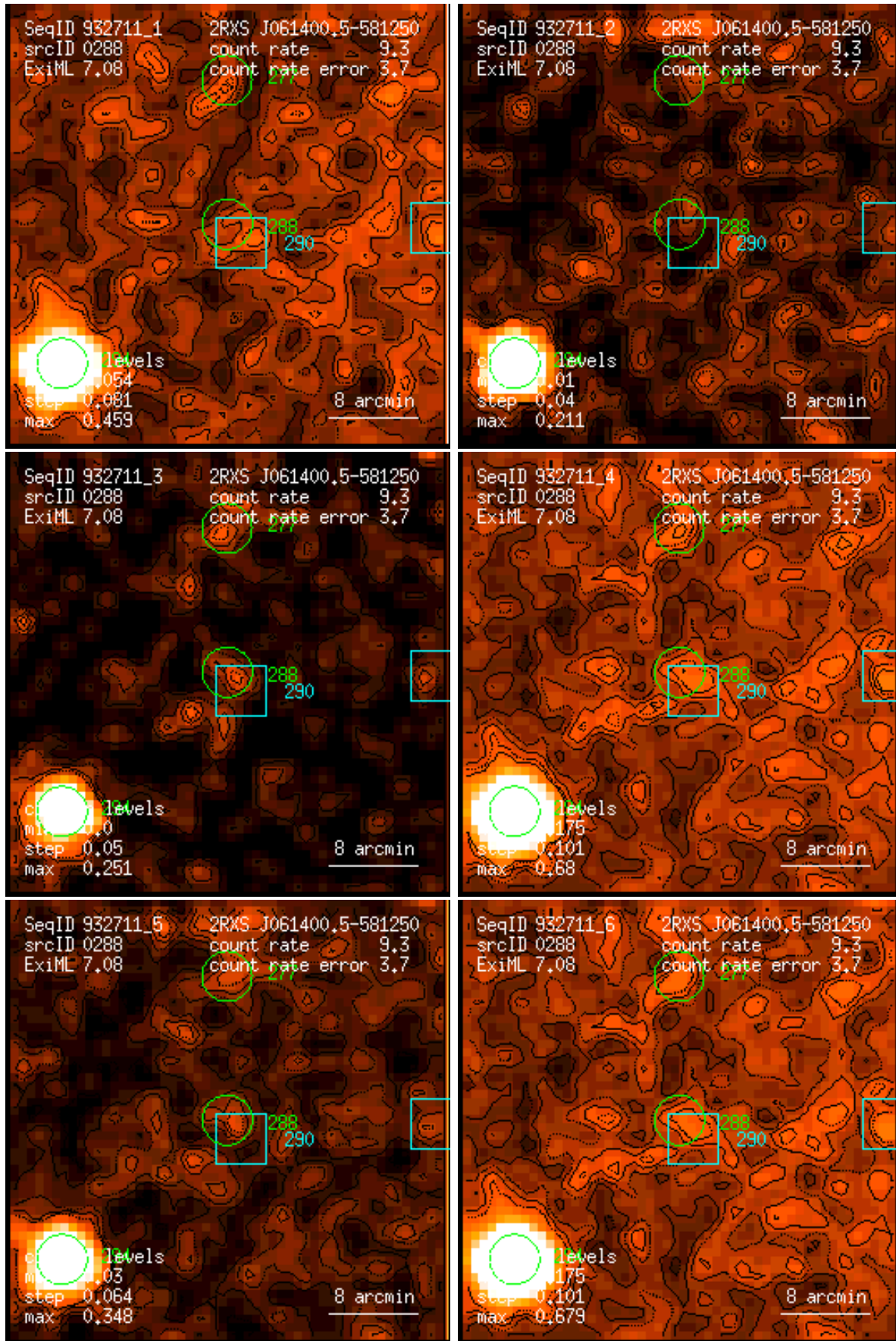
Figure 288: RASS 932711: detection 0288: band rate images, Gaussian filter: (1) PSPC channels 11 – 41, (2) 52 – 90, (3) 91 – 201, (4) 11 – 235, (5) 52 – 201, (6) 11 – 201. Broad band rates in counts/ks. Band rate contour levels in counts/ks/arcmin 2 .
