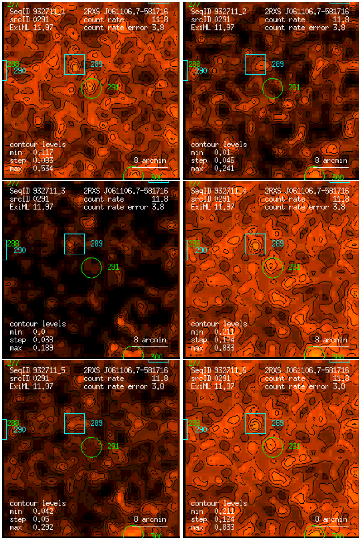
Figure 291: RASS 932711: detection 0291: band rate images, Gaussian filter: (1) PSPC channels 11 – 41, (2) 52 – 90, (3) 91 – 201, (4) 11 – 235, (5) 52 – 201, (6) 11 – 201. Broad band rates in counts/ks. Band rate contour levels in counts/ks/arcmin 2 .
