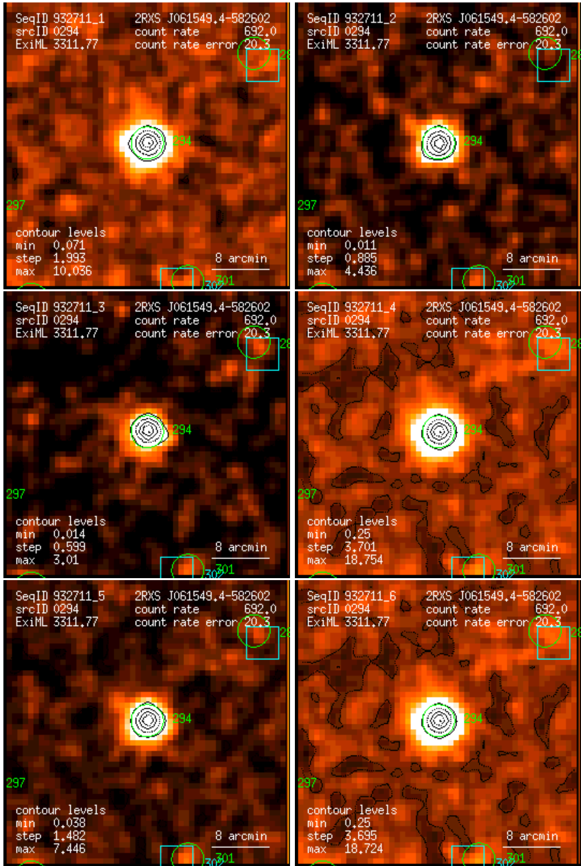
Figure 294: RASS 932711: detection 0294: band rate images, Gaussian filter: (1) PSPPC channels 11 – 41, (2) 52 – 90, (3) 91 – 201, (4) 11 – 235, (5) 52 – 201, (6) 11 – 201. Broad band rates in counts/ks. Band rate contour levels in counts/ks/arcmin 2 .
