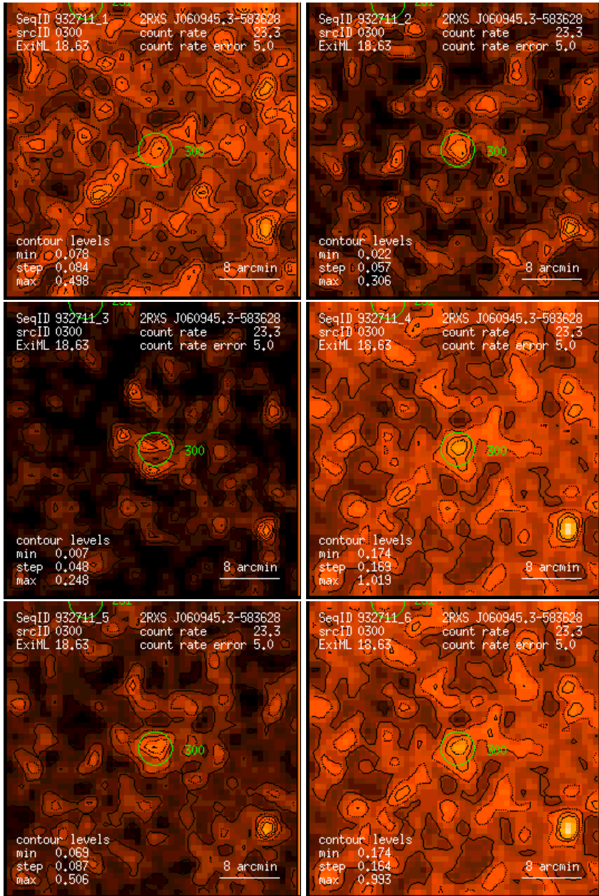
Figure 300: RASS 932711: detection 0300: band rate images, Gaussian filter: (1) PSPC channels 11 – 41, (2) 52 – 90, (3) 91 – 201, (4) 11 – 235, (5) 52 – 201, (6) 11 – 201. Broad band rates in counts/ks. Band rate contour levels in counts/ks/arcmin 2 .
