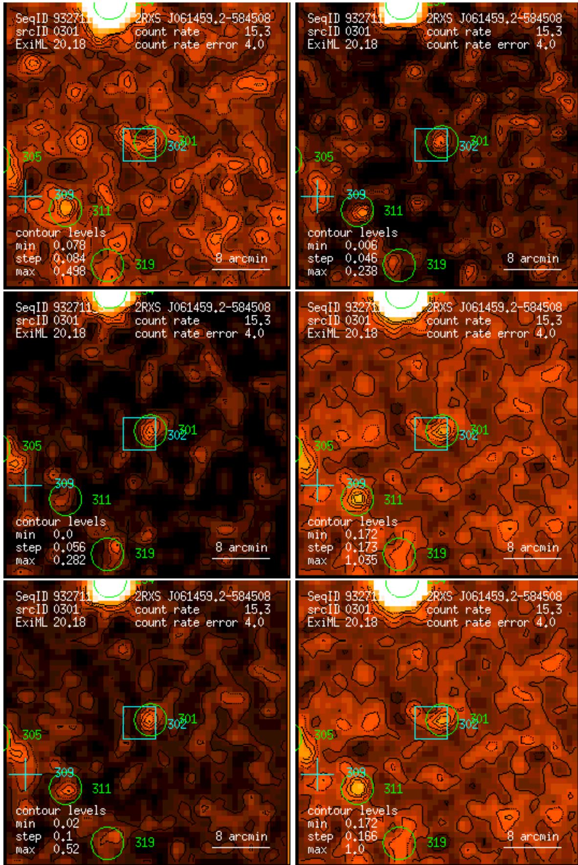
Figure 301: RASS 932711: detection 0301: band rate images, Gaussian filter: (1) PSPC channels 11 – 41, (2) 52 – 90, (3) 91 – 201, (4) 11 – 235, (5) 52 – 201, (6) 11 – 201. Broad band rates in counts/ks. Band rate contour levels in counts/ks/arcmin 2 .
