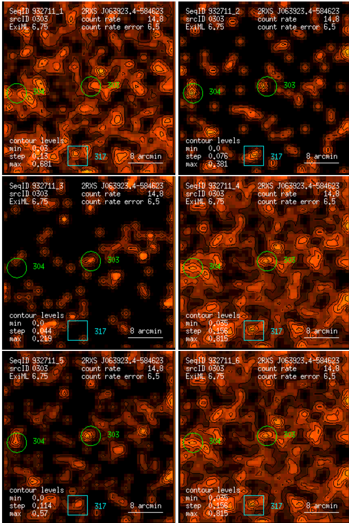
Figure 303: RASS 932711: detection 0303: band rate images, Gaussian filter: (1) PSPC channels 11 – 41, (2) 52 – 90, (3) 91 – 201, (4) 11 – 235, (5) 52 – 201, (6) 11 – 201. Broad band rates in counts/ks. Band rate contour levels in counts/ks/arcmin 2 .
