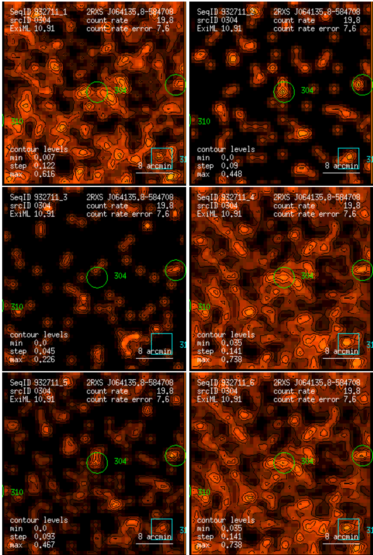
Figure 304: RASS 932711: detection 0304: band rate images, Gaussian filter: (1) PSPC channels 11 – 41, (2) 52 – 90, (3) 91 – 201, (4) 11 – 235, (5) 52 – 201, (6) 11 – 201. Broad band rates in counts/ks. Band rate contour levels in counts/ks/arcmin 2 .
