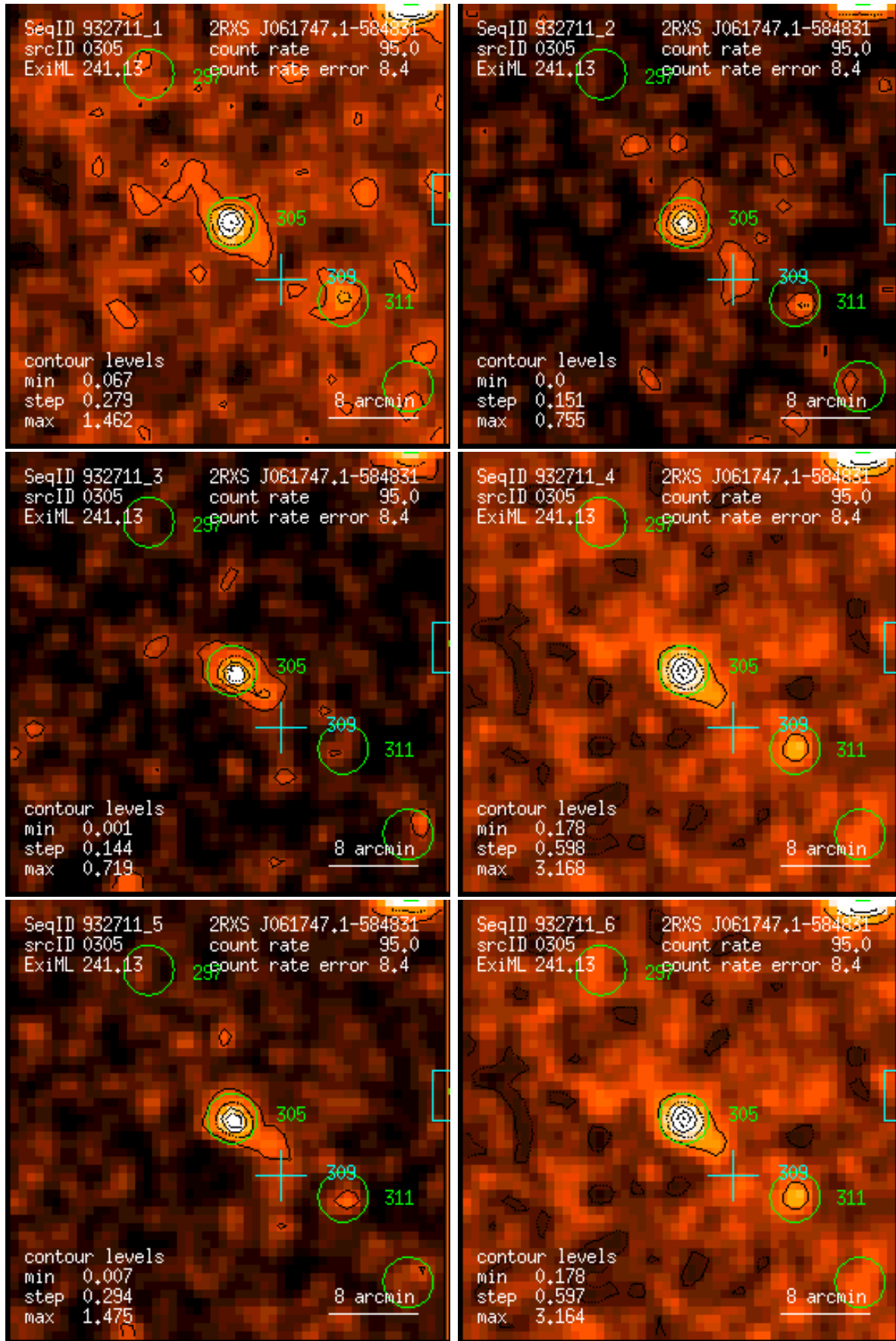
Figure 305: RASS 932711: detection 0305: band rate images, Gaussian filter: (1) PSPC channels 11 – 41, (2) 52 – 90, (3) 91 – 201, (4) 11 – 235, (5) 52 – 201, (6) 11 – 201. Broad band rates in counts/ks. Band rate contour levels in counts/ks/arcmin 2 .
