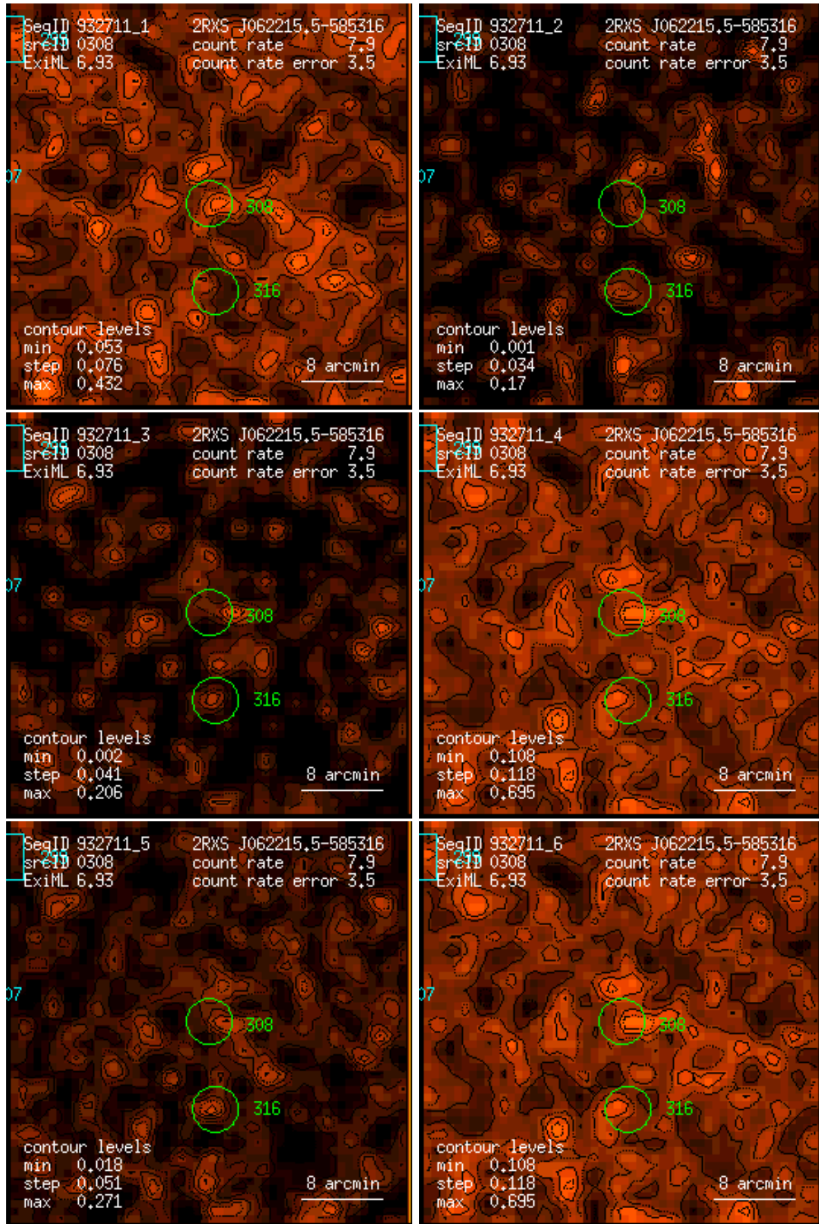
Figure 308: RASS 932711: detection 0308: band rate images, Gaussian filter: (1) PSPC channels 11 – 41, (2) 52 – 90, (3) 91 – 201, (4) 11 – 235, (5) 52 – 201, (6) 11 – 201. Broad band rates in counts/ks. Band rate contour levels in counts/ks/arcmin 2 .
