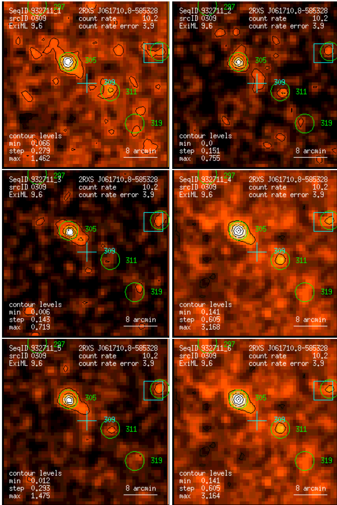
Figure 309: RASS 932711: detection 0309: band rate images, Gaussian filter: (1) PSPC channels 11 – 41, (2) 52 – 90, (3) 91 – 201, (4) 11 – 235, (5) 52 – 201, (6) 11 – 201. Broad band rates in counts/ks. Band rate contour levels in counts/ks/arcmin 2 .
