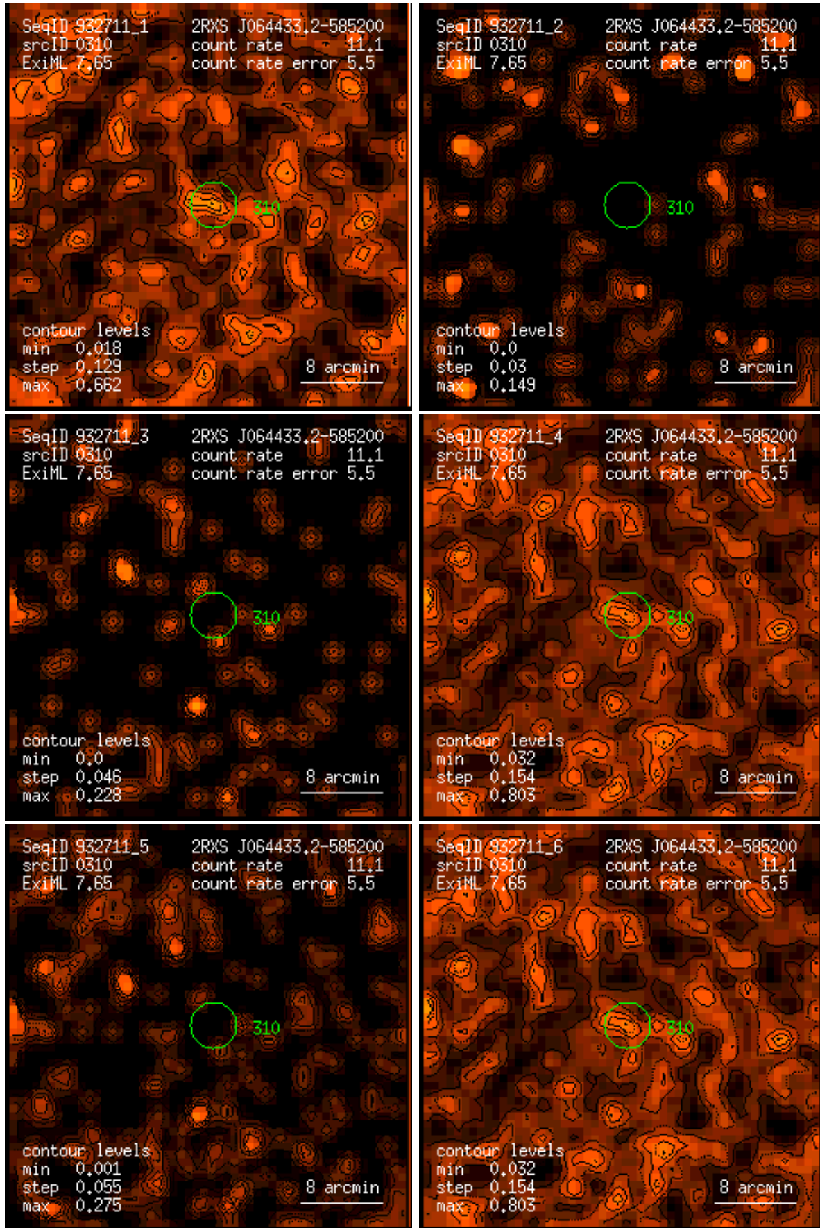
Figure 310: RASS 932711: detection 0310: band rate images, Gaussian filter: (1) PSPC channels 11 – 41, (2) 52 – 90, (3) 91 – 201, (4) 11 – 235, (5) 52 – 201, (6) 11 – 201. Broad band rates in counts/ks. Band rate contour levels in counts/ks/arcmin 2 .
