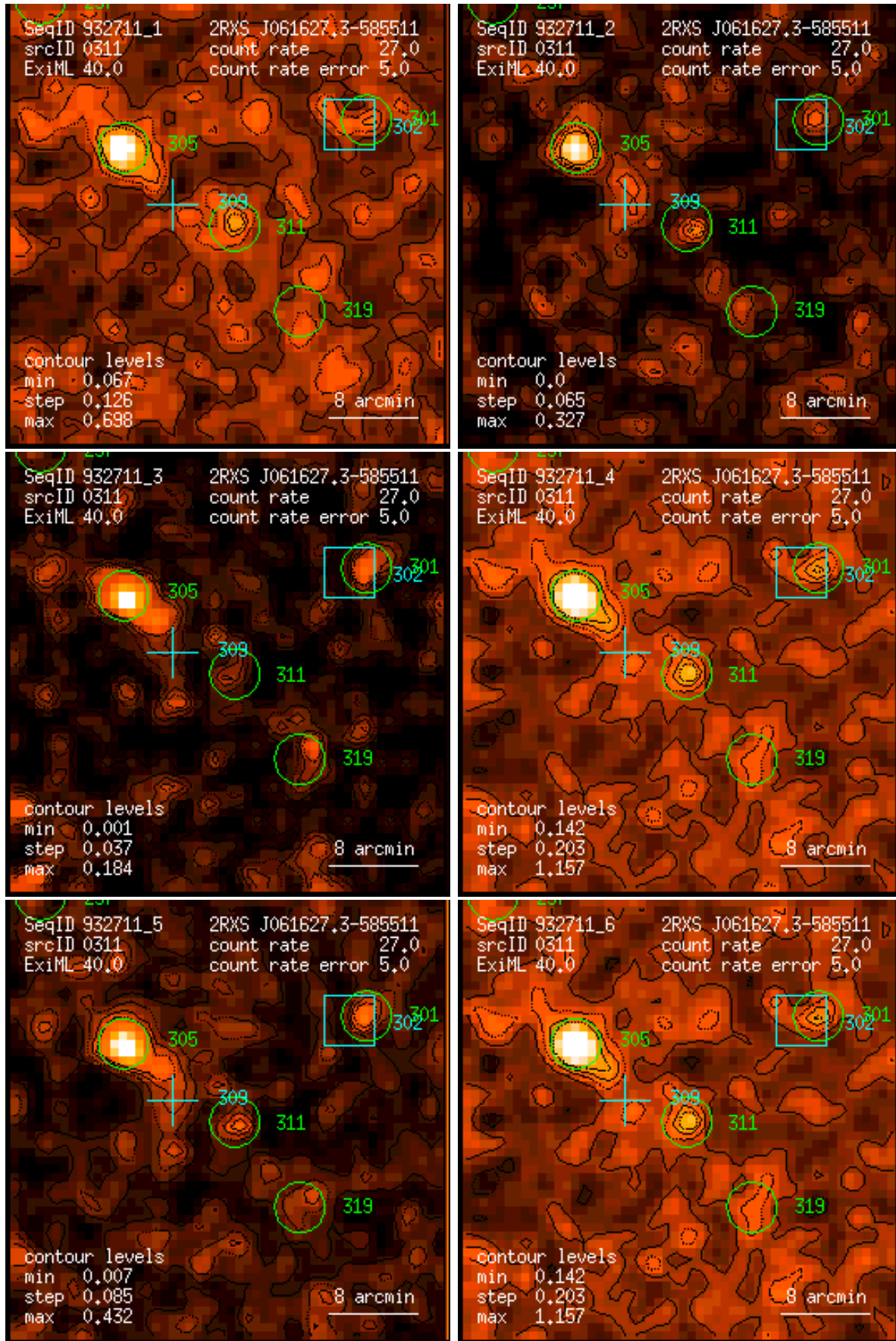
Figure 311: RASS 932711: detection 0311: band rate images, Gaussian filter: (1) PSPC channels 11 – 41, (2) 52 – 90, (3) 91 – 201, (4) 11 – 235, (5) 52 – 201, (6) 11 – 201. Broad band rates in counts/ks. Band rate contour levels in counts/ks/arcmin 2 .
